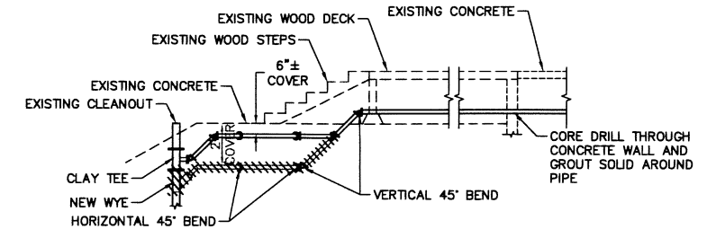
FORCE MAIN PROFILE NOT TO SCALE
