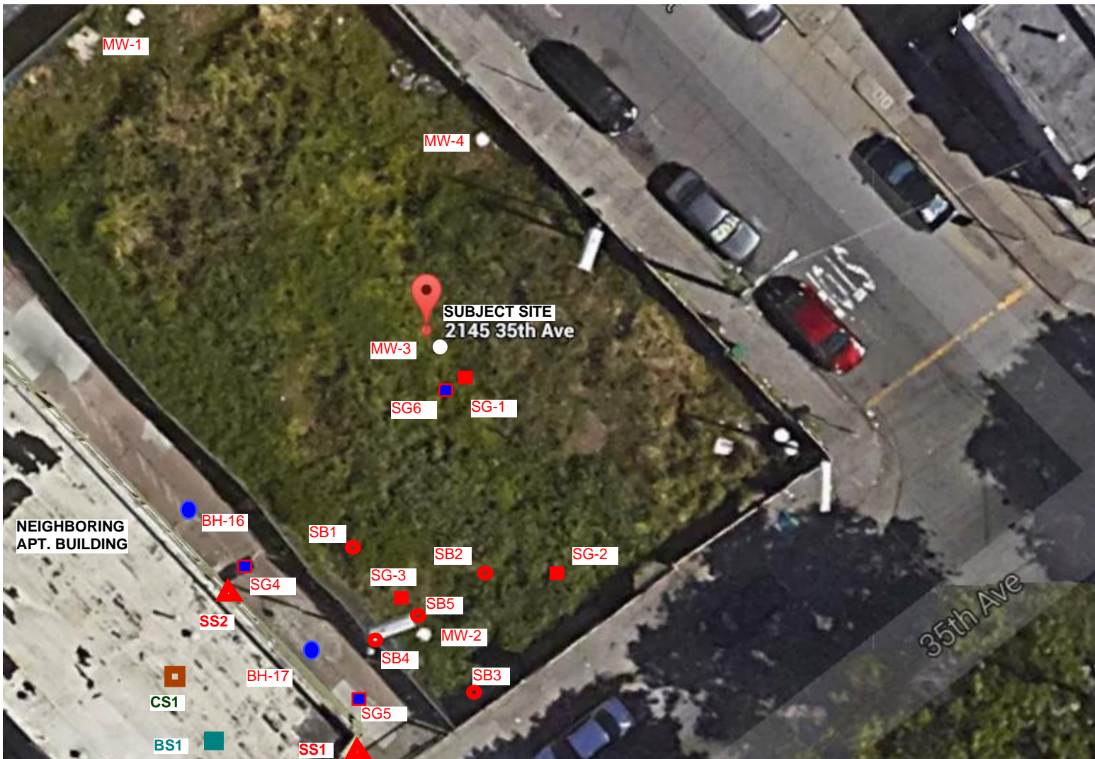
Figure 2- Planned Locations of the Sub-Slab Soil Gas and Crawl Space Air Sampling
