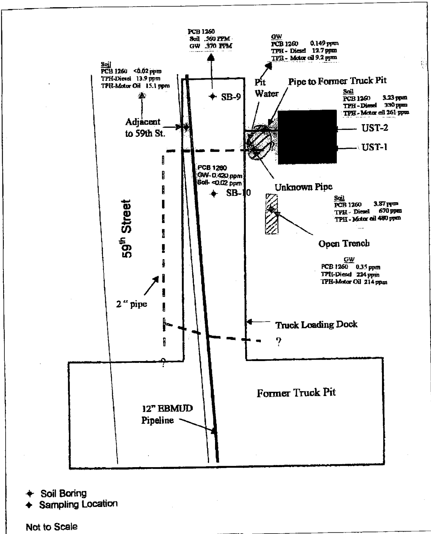
Figure 4: Connector Pipe and Soil Boring Locations
