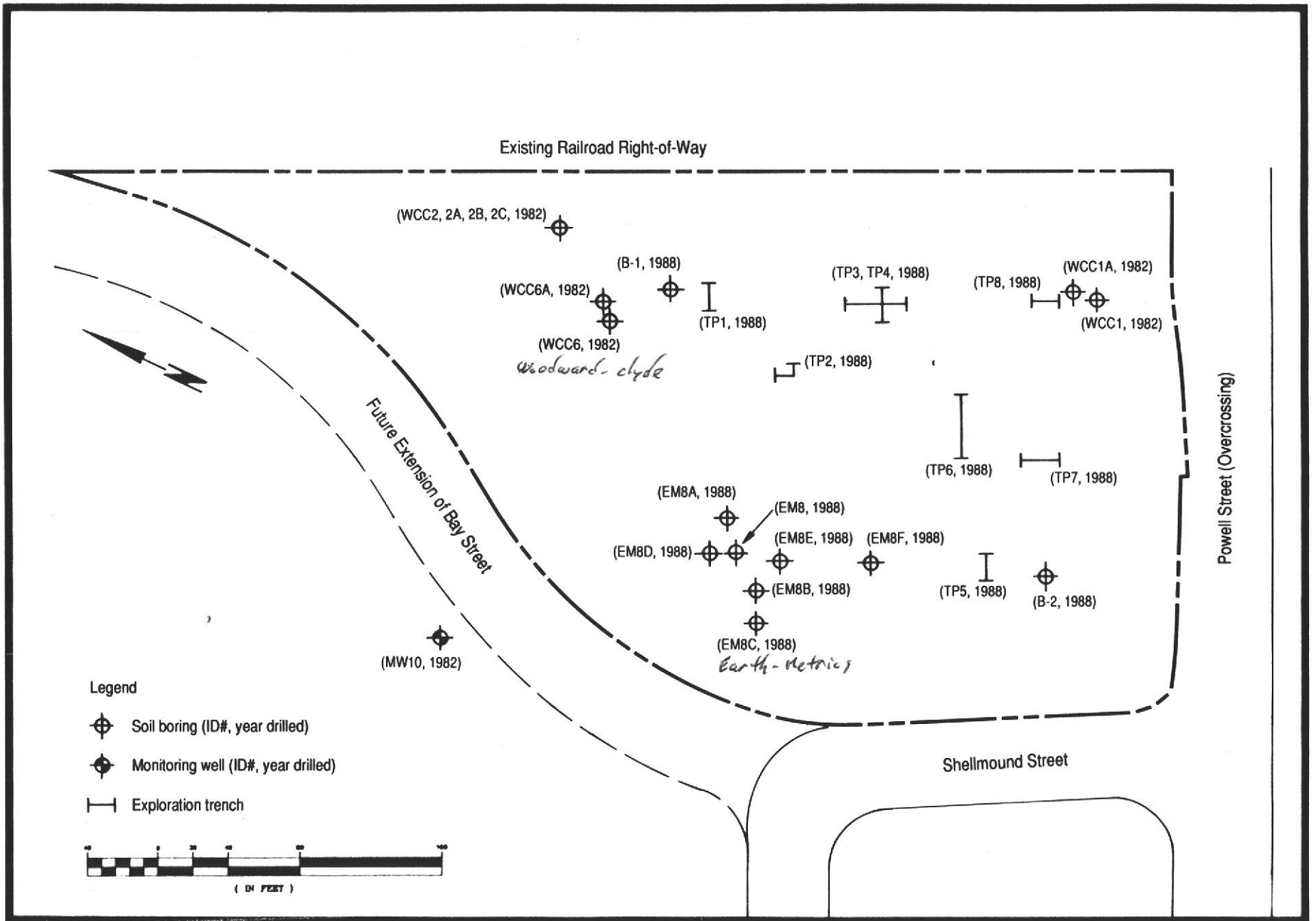
Plan of Borings and Explorations on Site of Another Tree Emeryville Project
