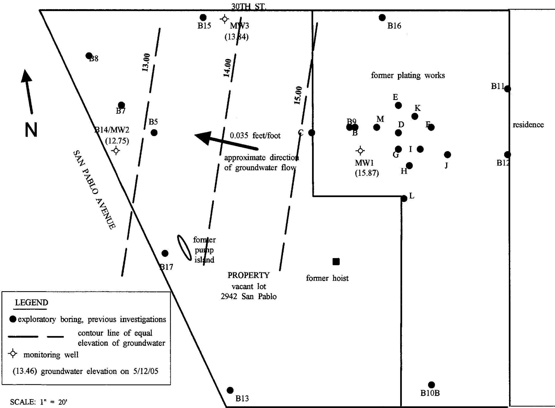
Figure 2 - Potentiometric Surface on May 12, 2005
