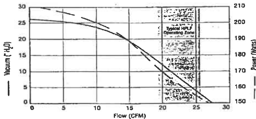
Figure 6 - Regenerative Blower Performance Curve
