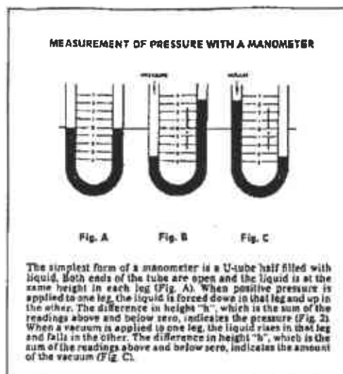
Figure 7 - Simple U-Tube Manometer
