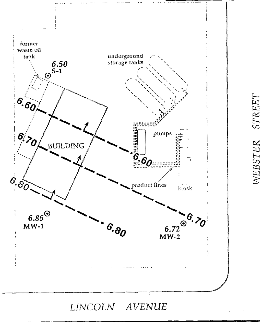
Figure 2. Ground Water Elevation Contours - April 23, 1992 - Shell Service Station WIC #204-0072-0403, 1601 Webster Street, Alameda, California
