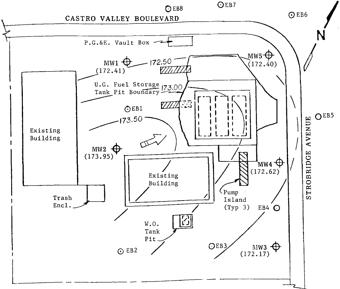
SITE PLAN
