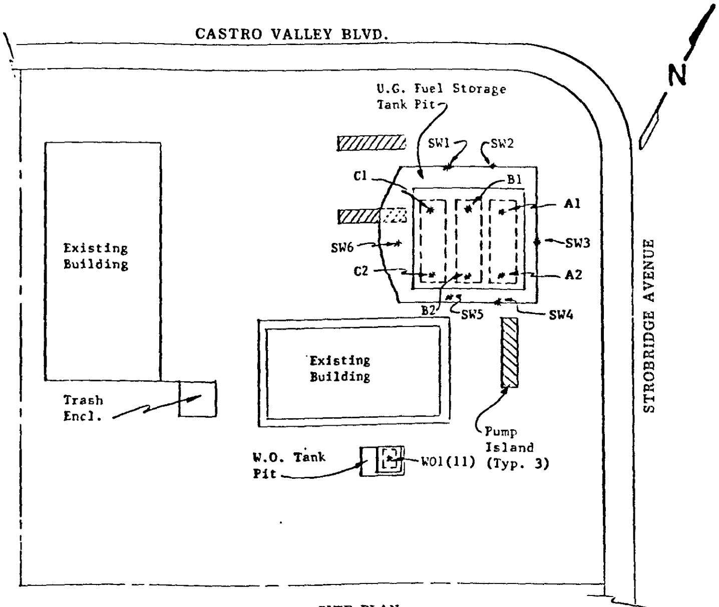
SITE PLAN
