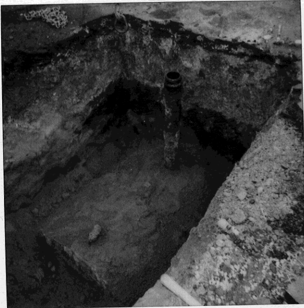
Waste oil tank + pit - E. wall shown 20009 Meekland Av. Hayward 10-16-90
