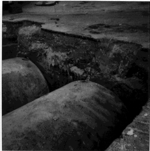
North tank wall 20009 Meekland Av. Hayward. Hoang's Auto Care 10/16/90
