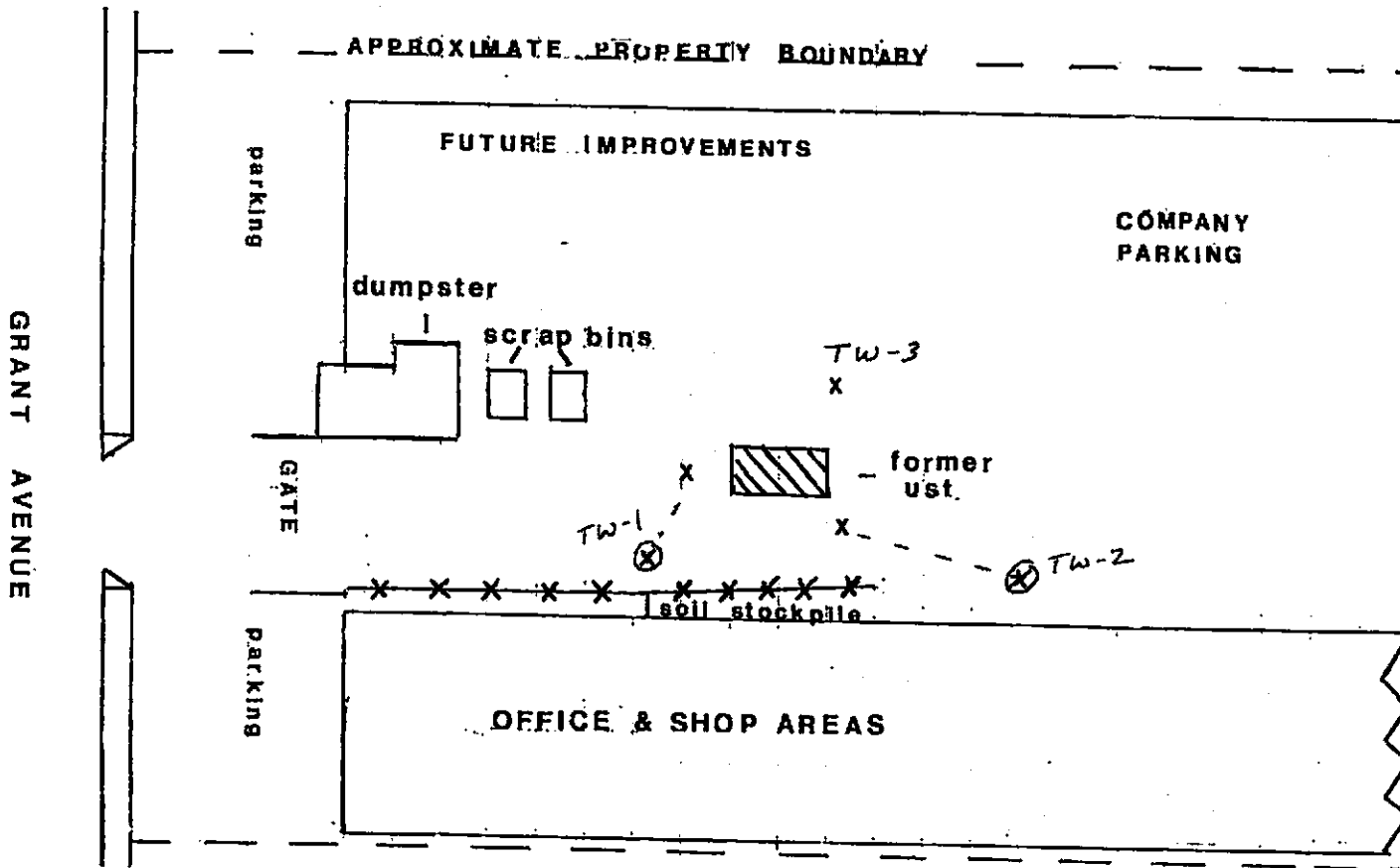
FIGURE 2. PROPOSED TEMPORARY WELL LOCATION MAP - FEBRUARY 1996 - 2584 GRANT AVENUE, SAN LORENZO, CALIFORNIA
