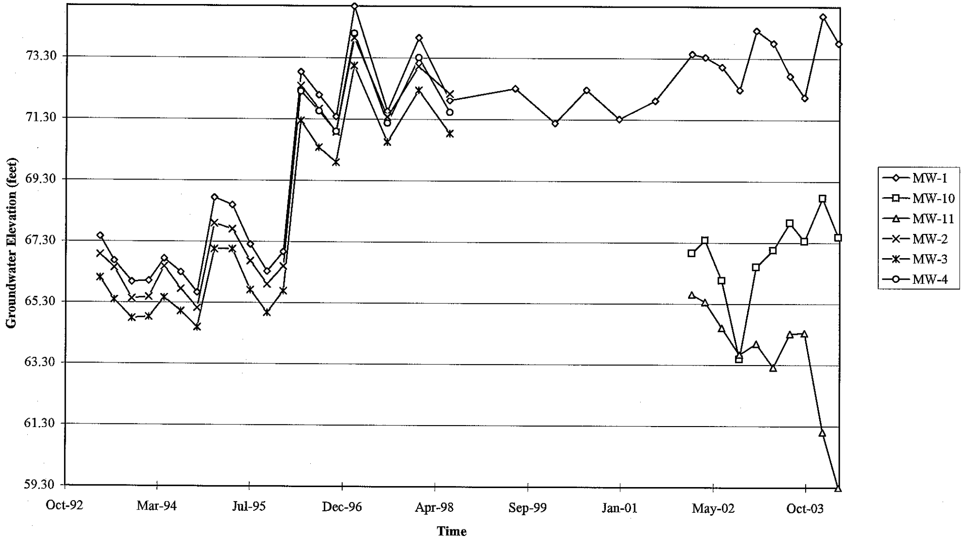
Graph 3 Hydrograph 76 Station 1871
