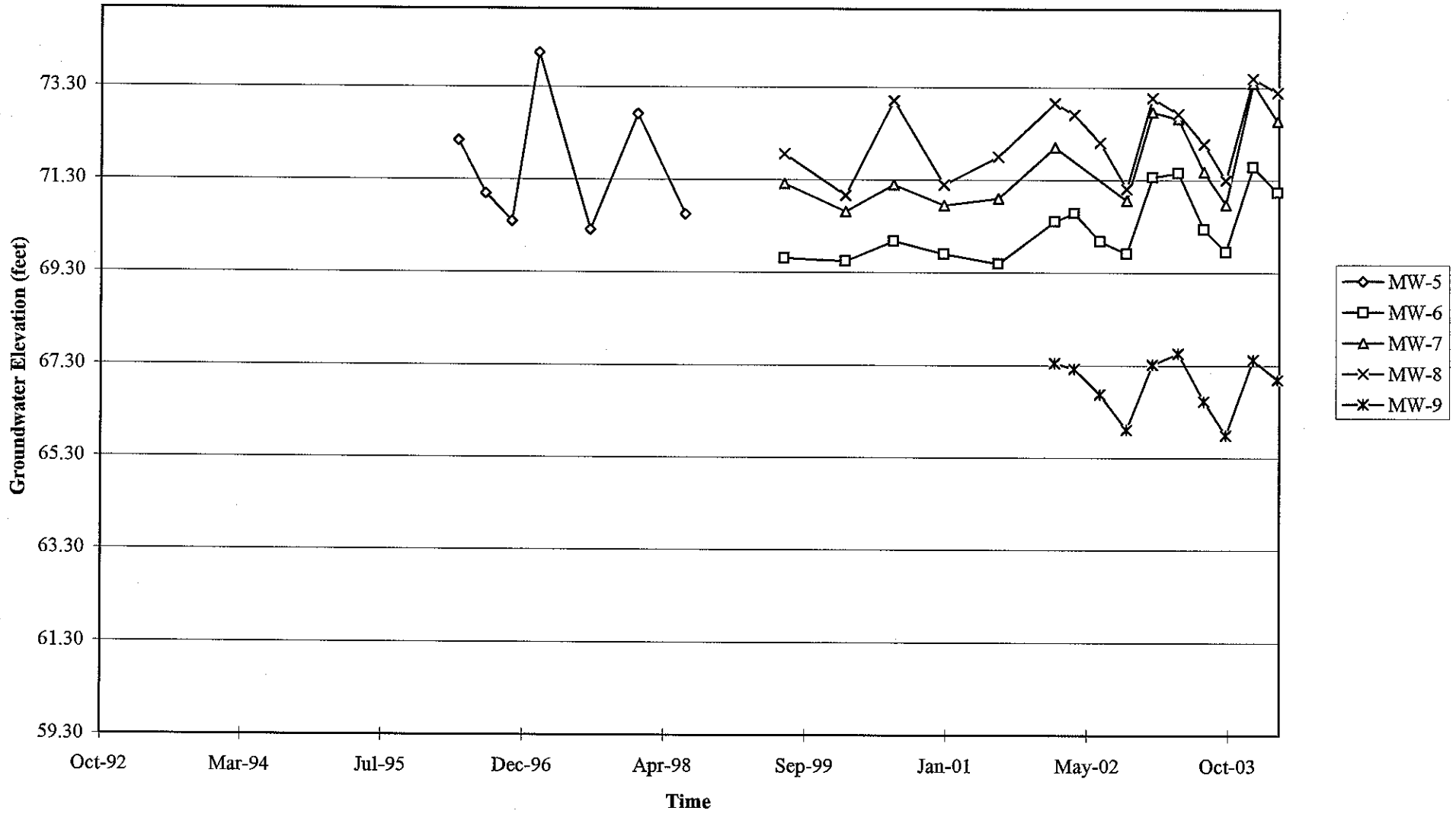
Graph 4 Hydrograph 76 Station 1871
