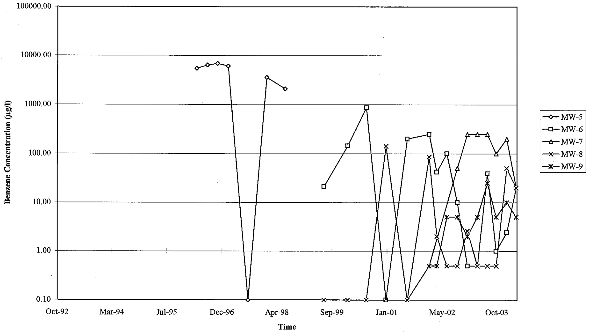
Graph 2 Benzene Concentrations vs. Time 76 Station 1871
