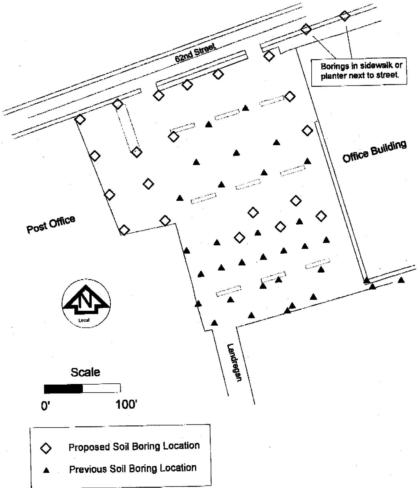
Figure 6: Locations of Proposed Soil Borings
