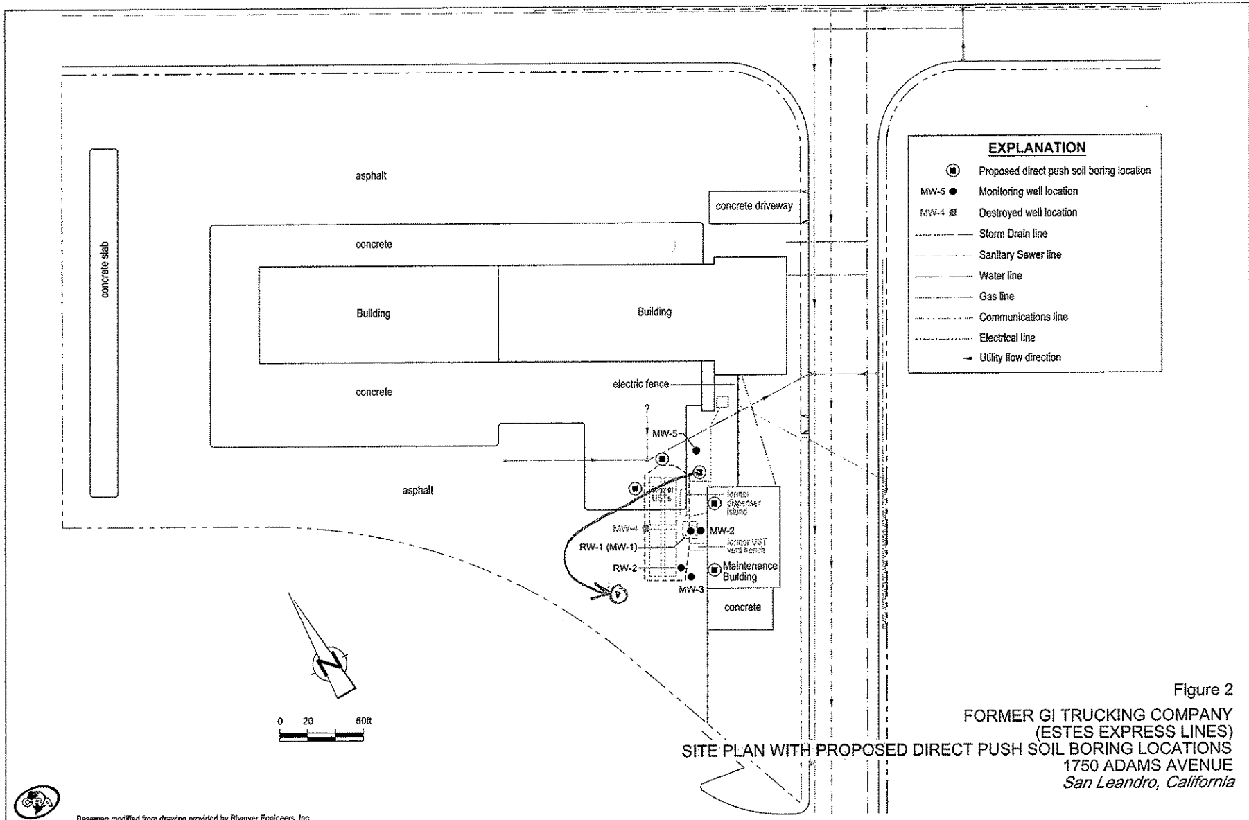
Figure 2 - Modified Soil Boring Location
