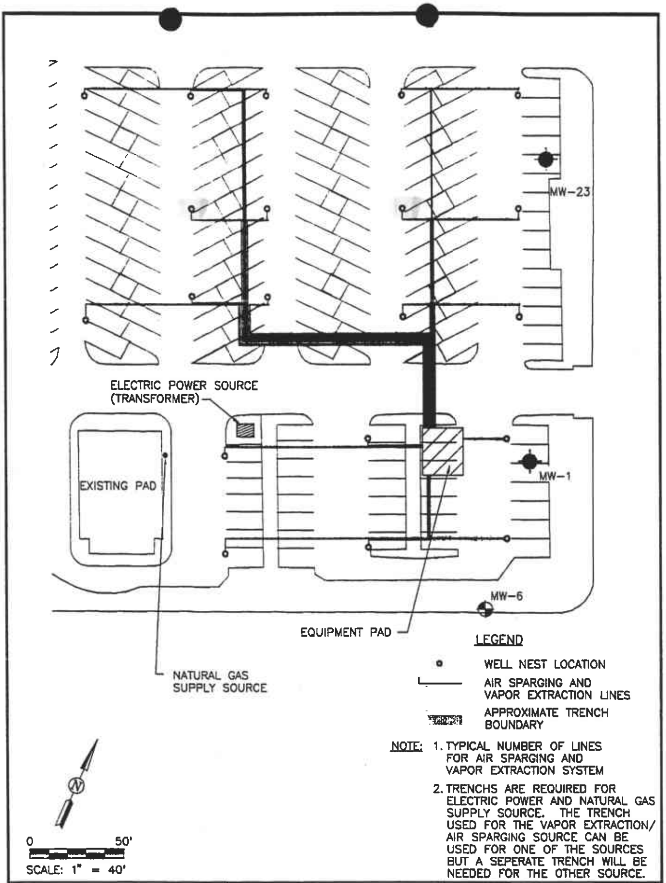
Figure 4 AIR SPARGING AND VAPOR EXTRACTION LAYOUT FOR SAFEWAY SITE BEACON STATION No. 604
