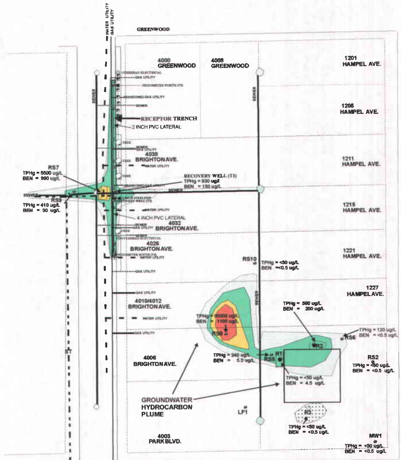
FIGURE 5 GROUNDWATER PLUME 03/13/03
