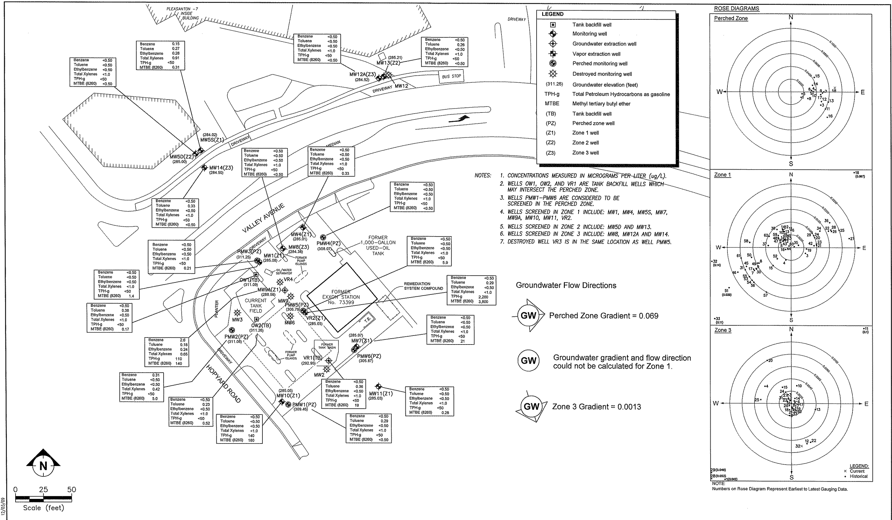
FILENAME: 402009.DWG 12/03/09 ETIC ENGINEERING SITE MAP SHOWING GROUNDWATER ELEVATIONS, ANALYTICAL RESULTS, AND ROSE DIAGRAMS FORMER EXXON RS 73399 2991 HOPYARD ROAD, PLEASANTON, CALIFORNIA 9 AND 10 NOVEMBER 2009 FIGURE: 1
