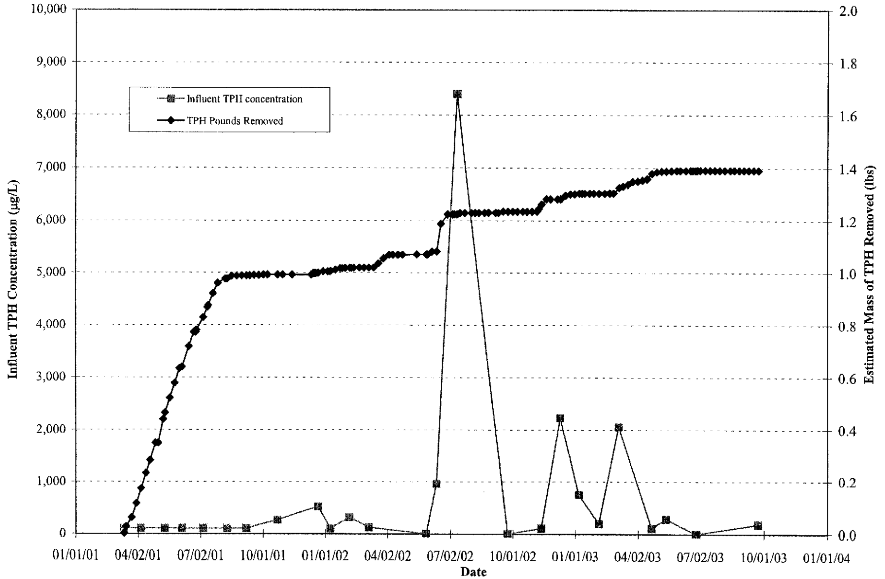
Figure 2: Influent TPH Concentrations and Estimated Mass of TPH Removed by Groundwater Extraction Former Exxon RS 7-3399, 2991 Hopyard Road, Pleasanton, CA
