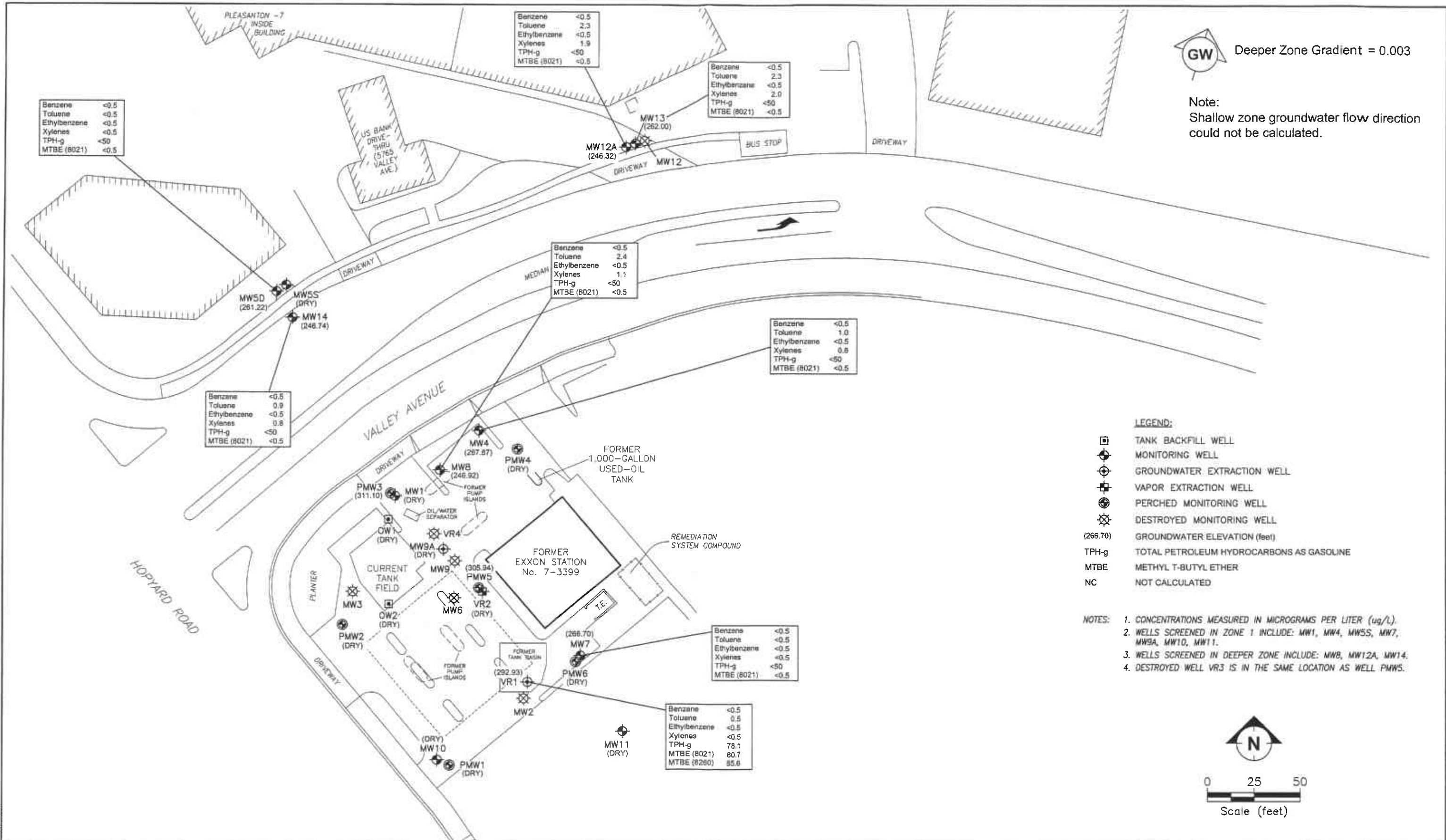
SITE PLAN SHOWING GROUNDWATER ELEVATIONS AND ANALYTICAL RESULTS FORMER EXXON RS 7-3399 2991 HOPYARD ROAD, PLEASANTON, CALIFORNIA 22 SEPTEMBER 2003
