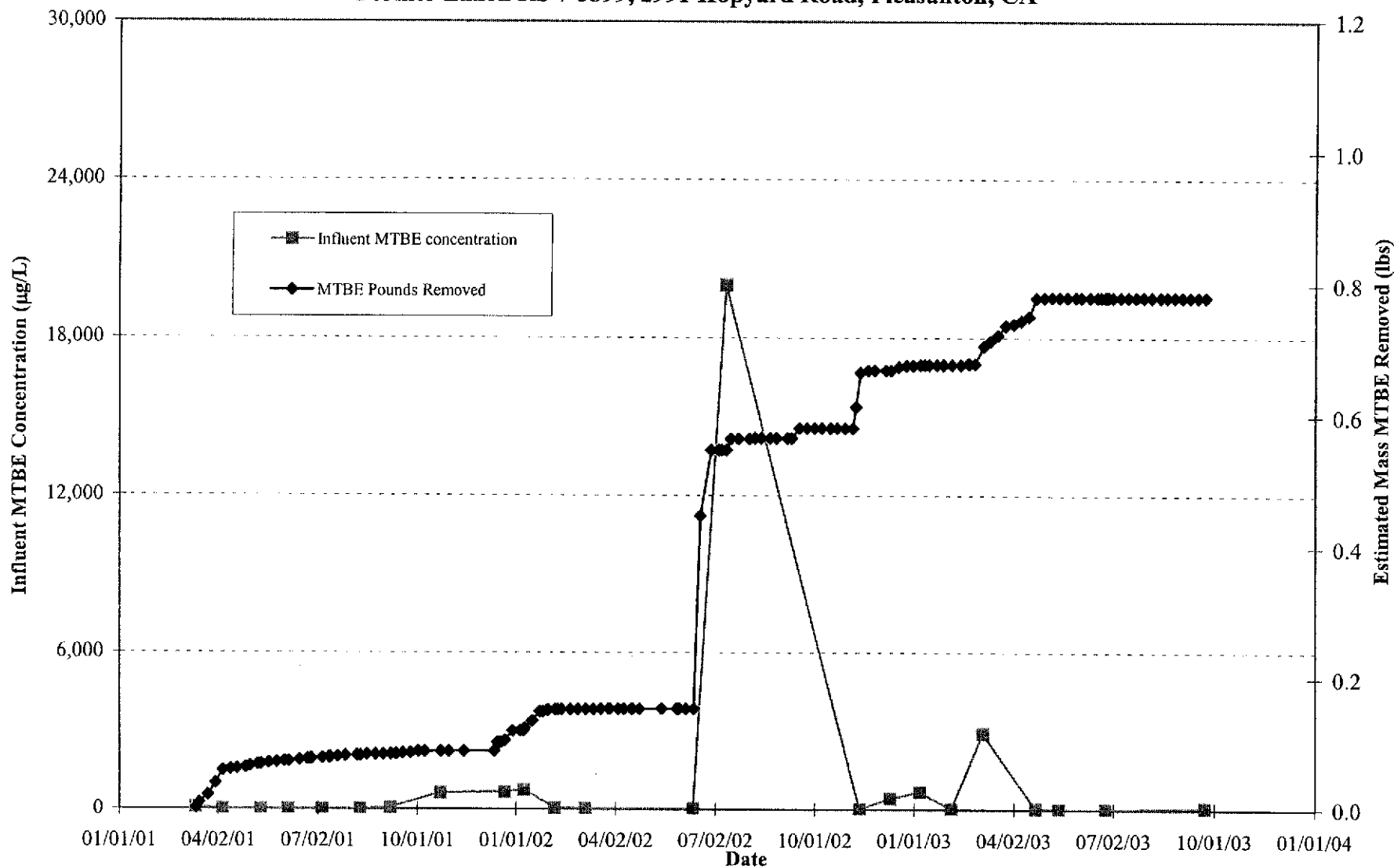
Figure 4: Influent MTBE Concentrations and Estimated Mass of MTBE Removed by Groundwater Extraction Former Exxon RS 7-3399, 2991 Hopyard Road, Pleasanton, CA
