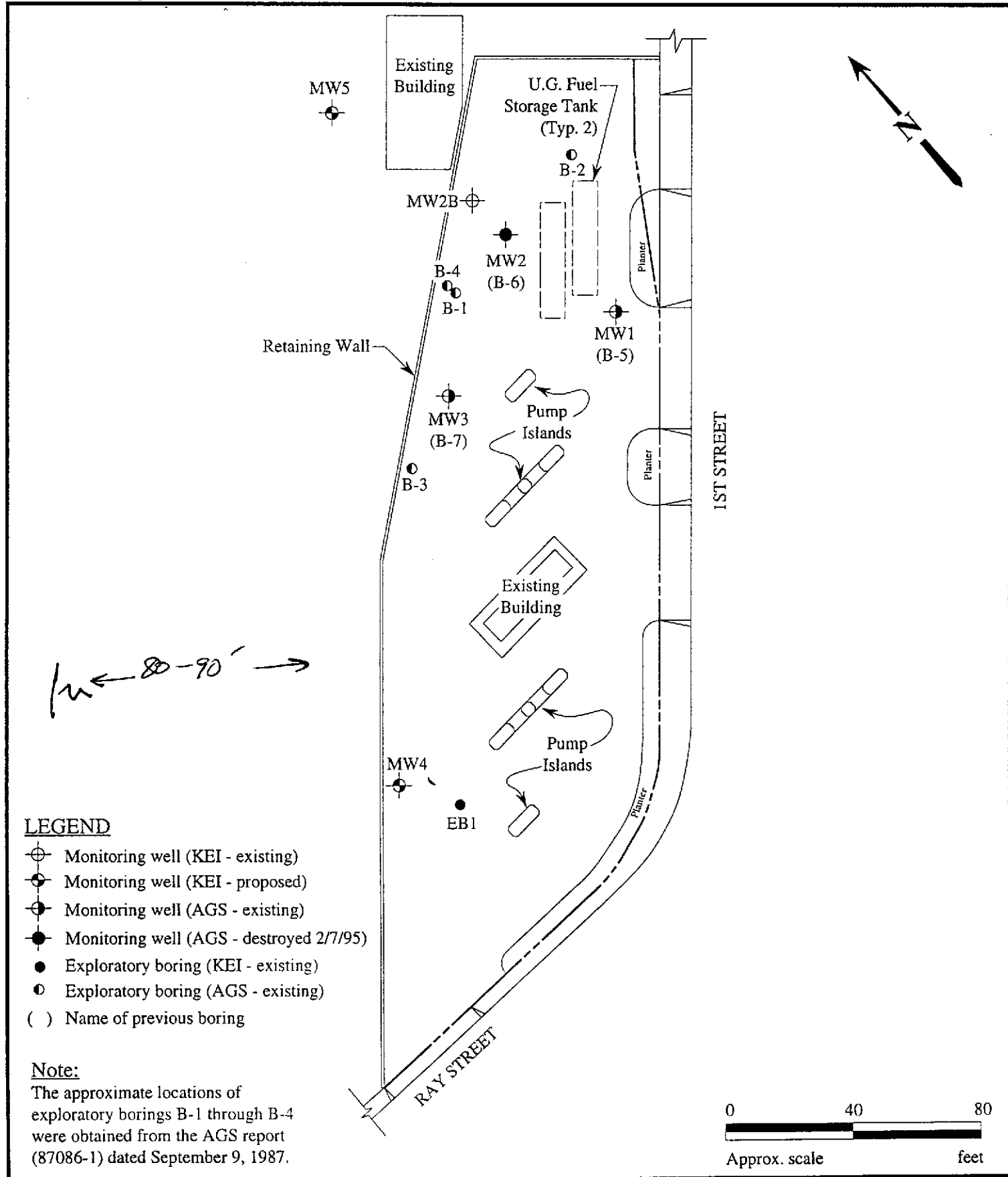
MONITORING WELL AND EXPLORATORY BORING LOCATION MAP
