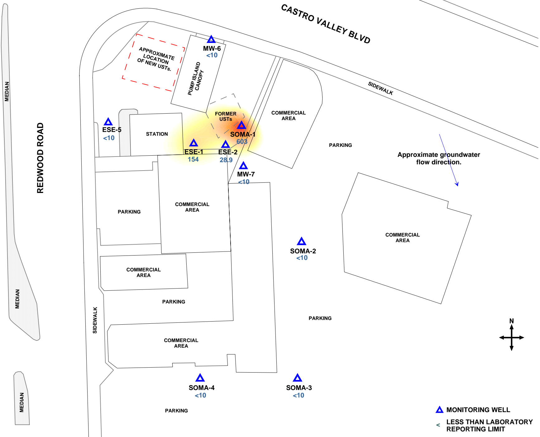
Figure 6: Contour map of TBA concentrations in groundwater. October 19, 2006.
