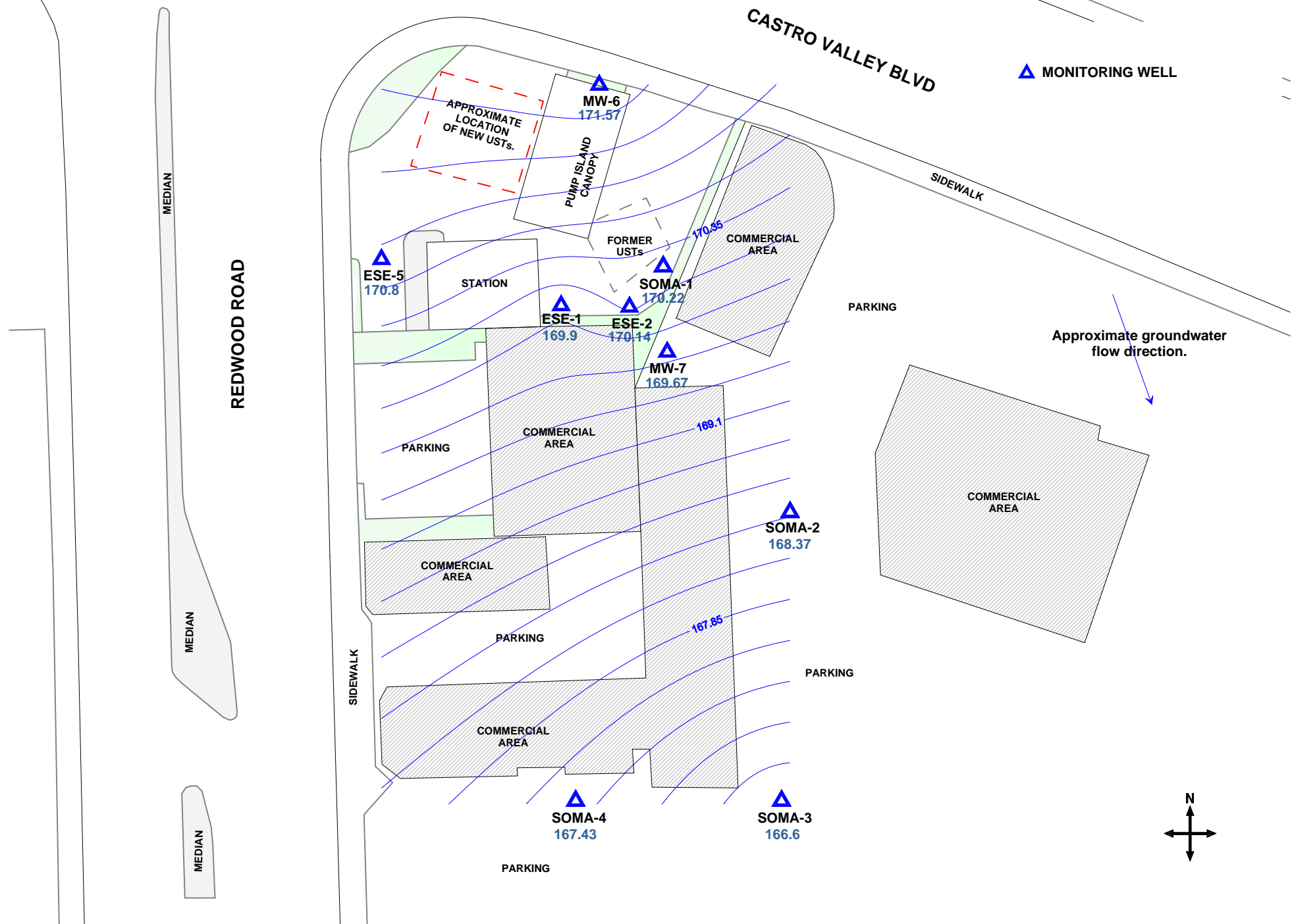
Figure 3: Groundwater elevation contour map in feet. October 19, 2006.
