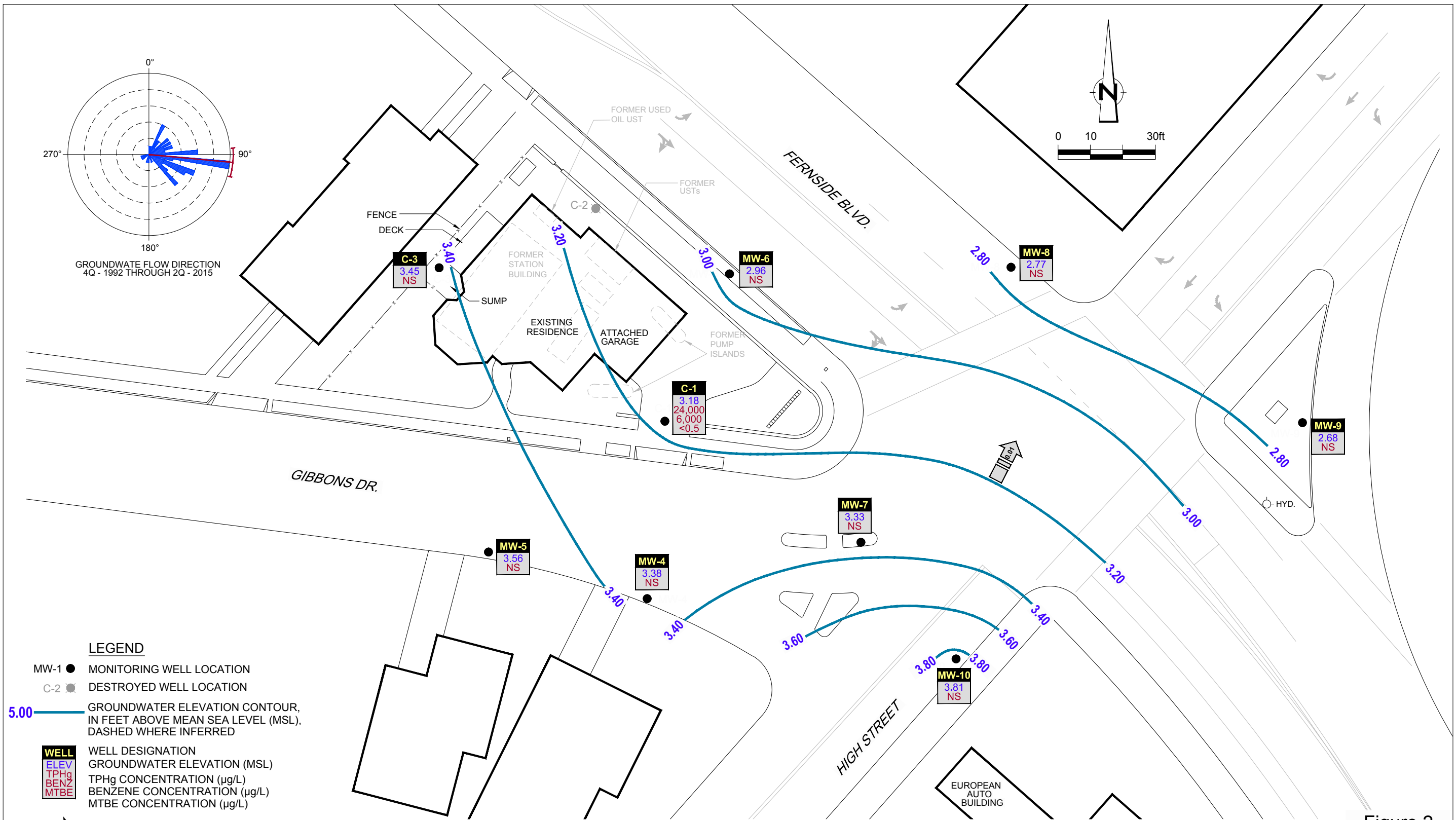
Figure 2 GROUNDWATER ELEVATION AND HYDROCARBON CONCENTRATION MAP FORMER CHEVRON SERVICE STATION 91153 3135 GIBBONS DRIVE (3126 FERNSIDE BLVD) Alameda, California June 18, 2015
