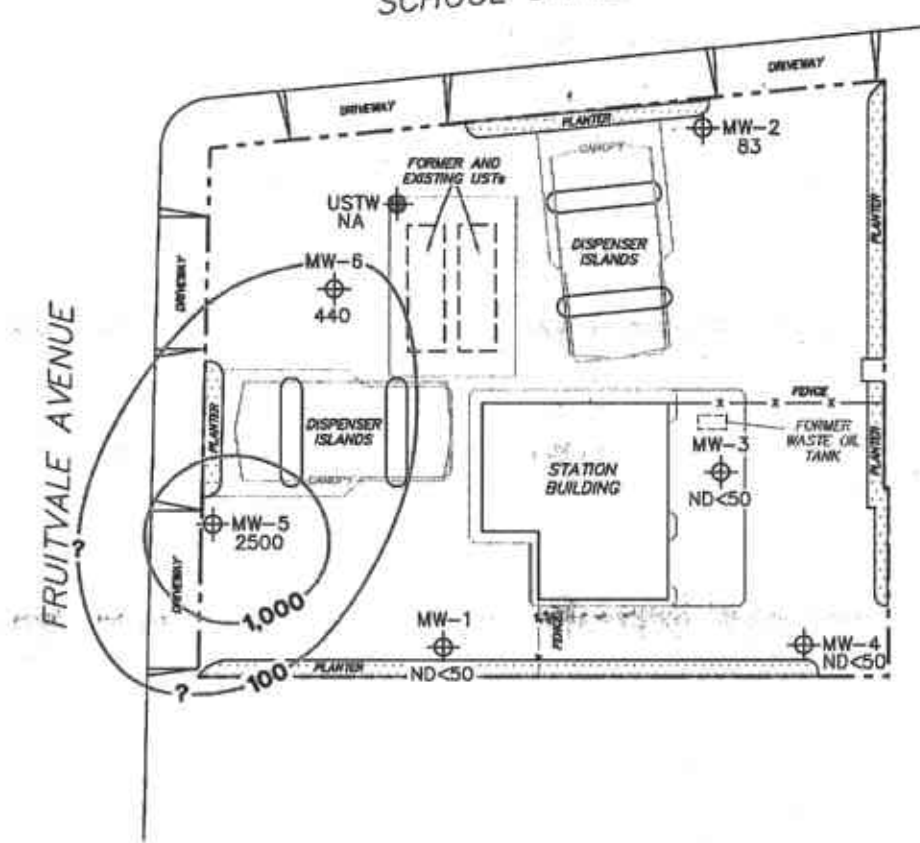
DISSOLVED-PHASE TPPH CONCENTRATION MAP September 26, 2005
