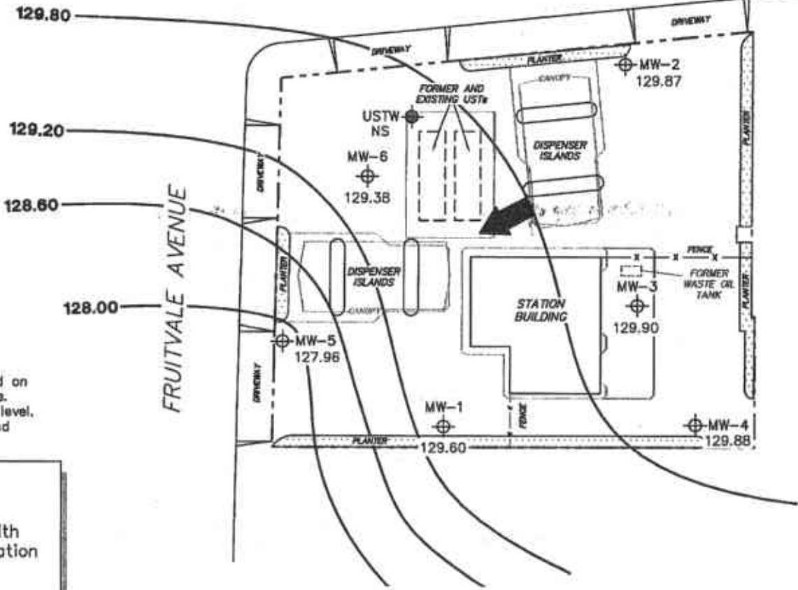
GROUNDWATER ELEVATION CONTOUR MAP September 26, 2005
