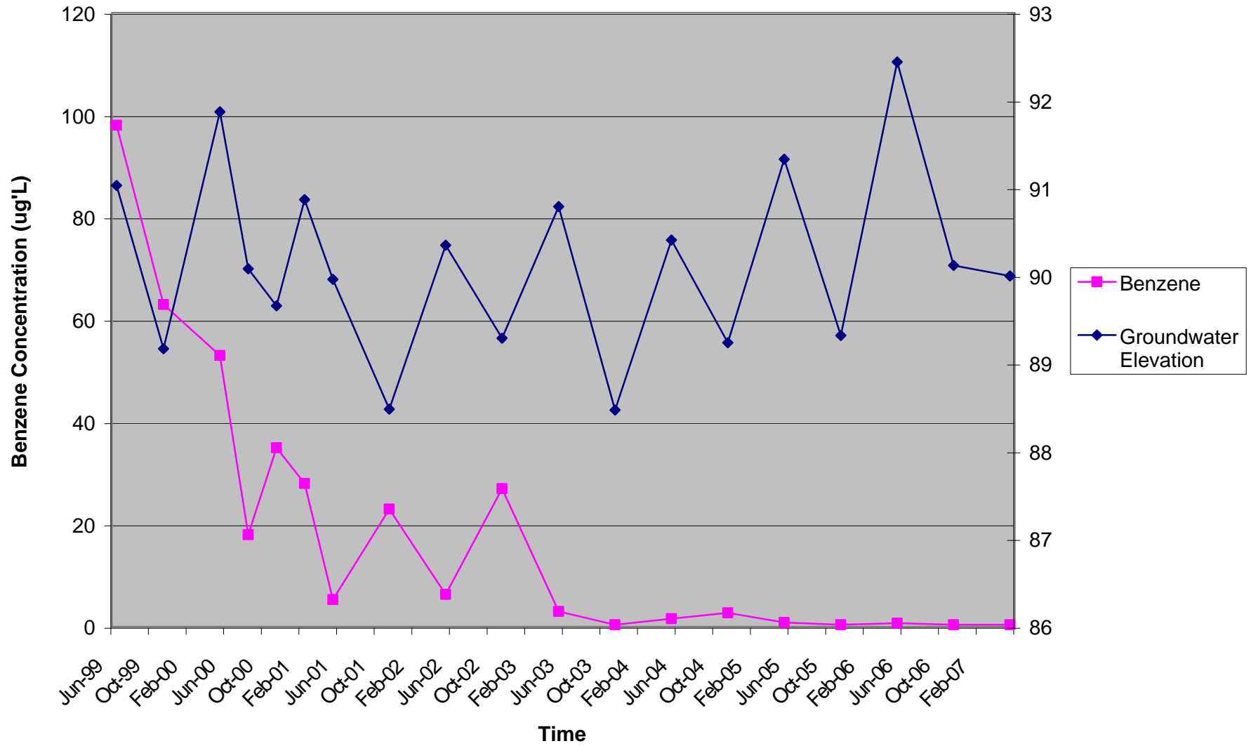
Figure 6: Concentration of Benzene Since June 1999 in MW-3
