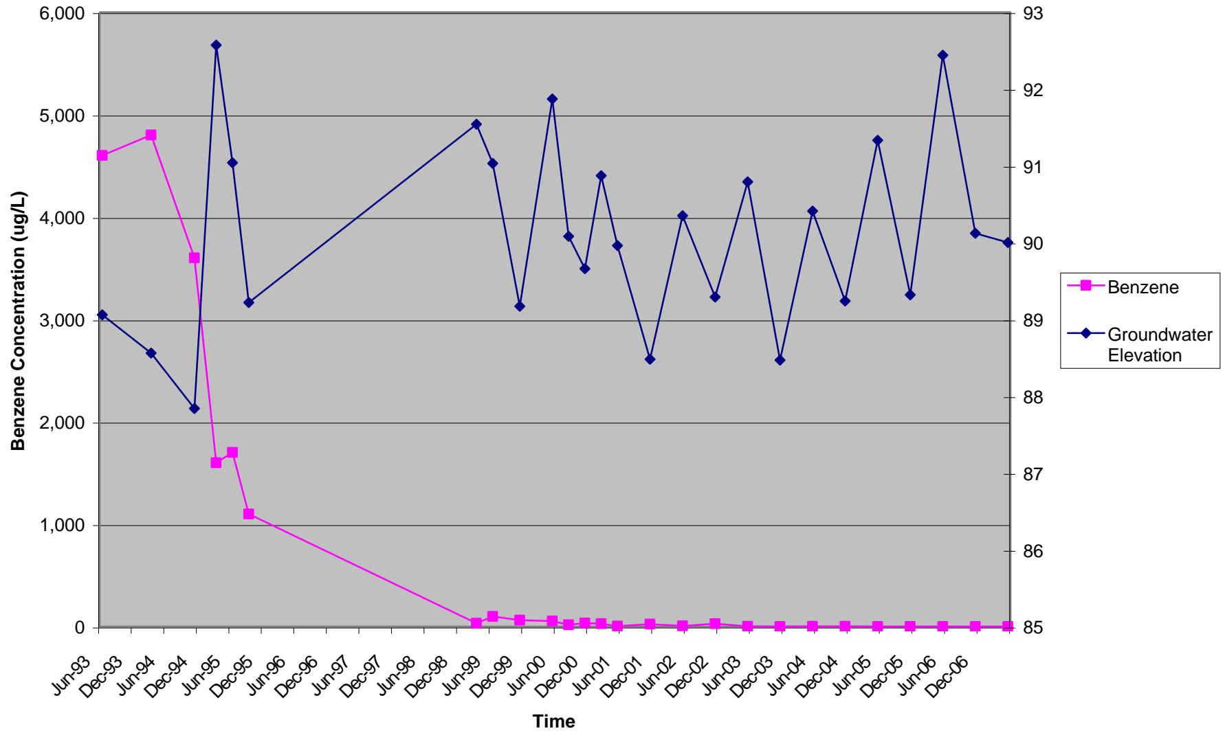
Figure 4: Benzene Concentration Over Time in MW-3
