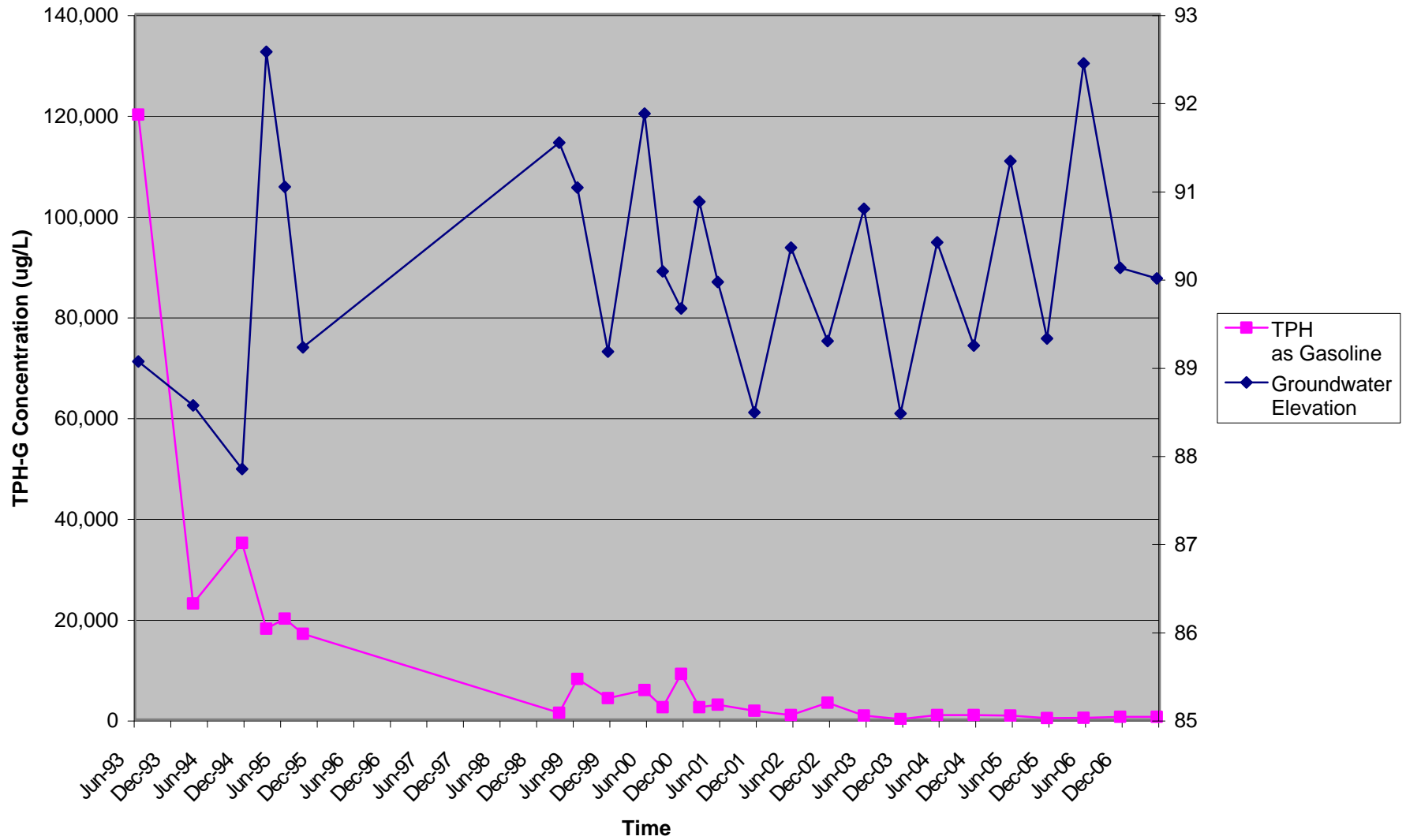
Figure 3: TPH as Gasoline Concentration Over Time in MW-3
