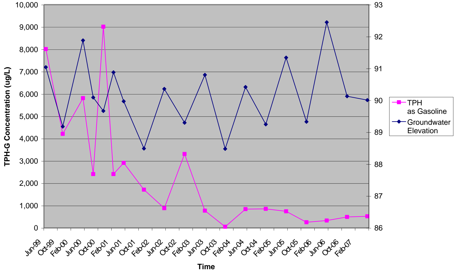
Figure 5: Concentration of TPH as Gasoline Since June 1999 in MW-3
