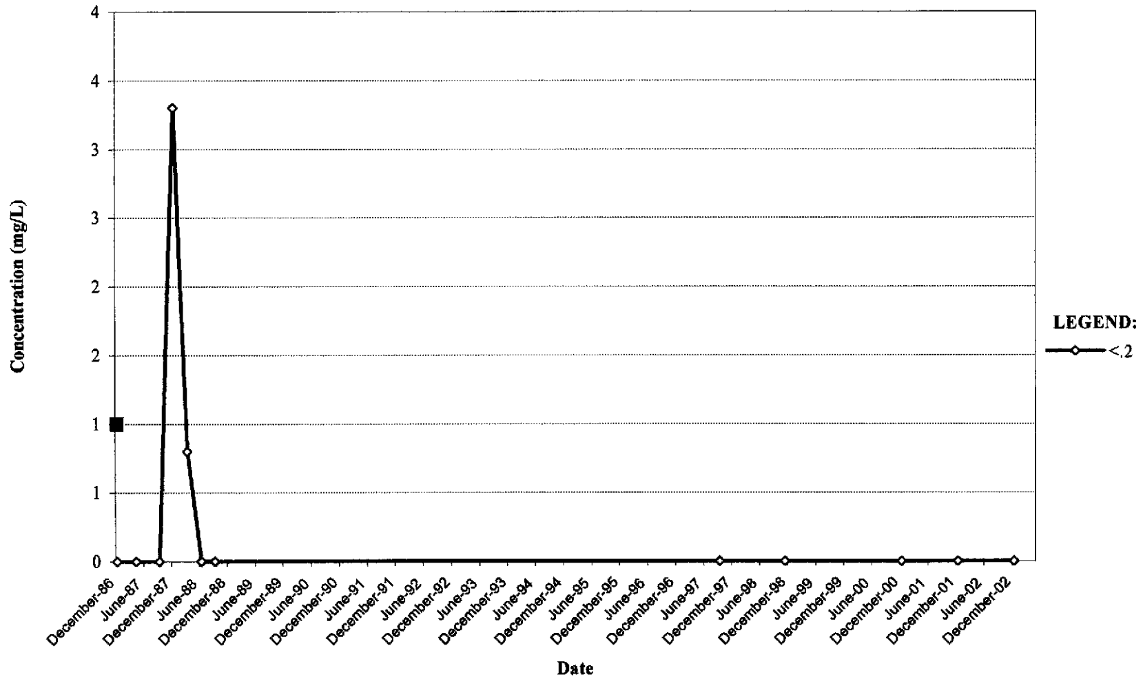
Trend Plot for Benzene Well MW-15
