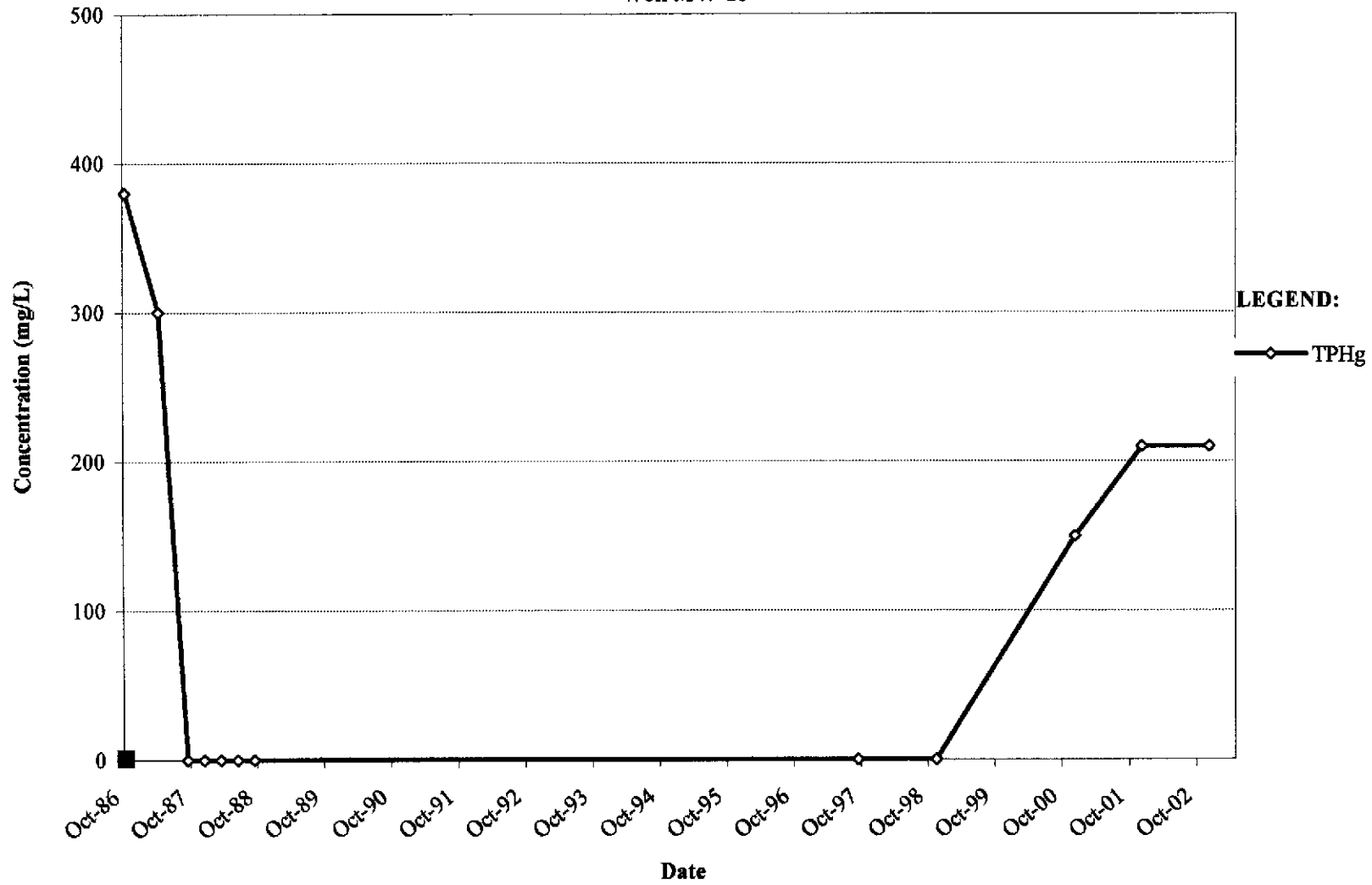
Trend Plot for TPHg Well MW-10
