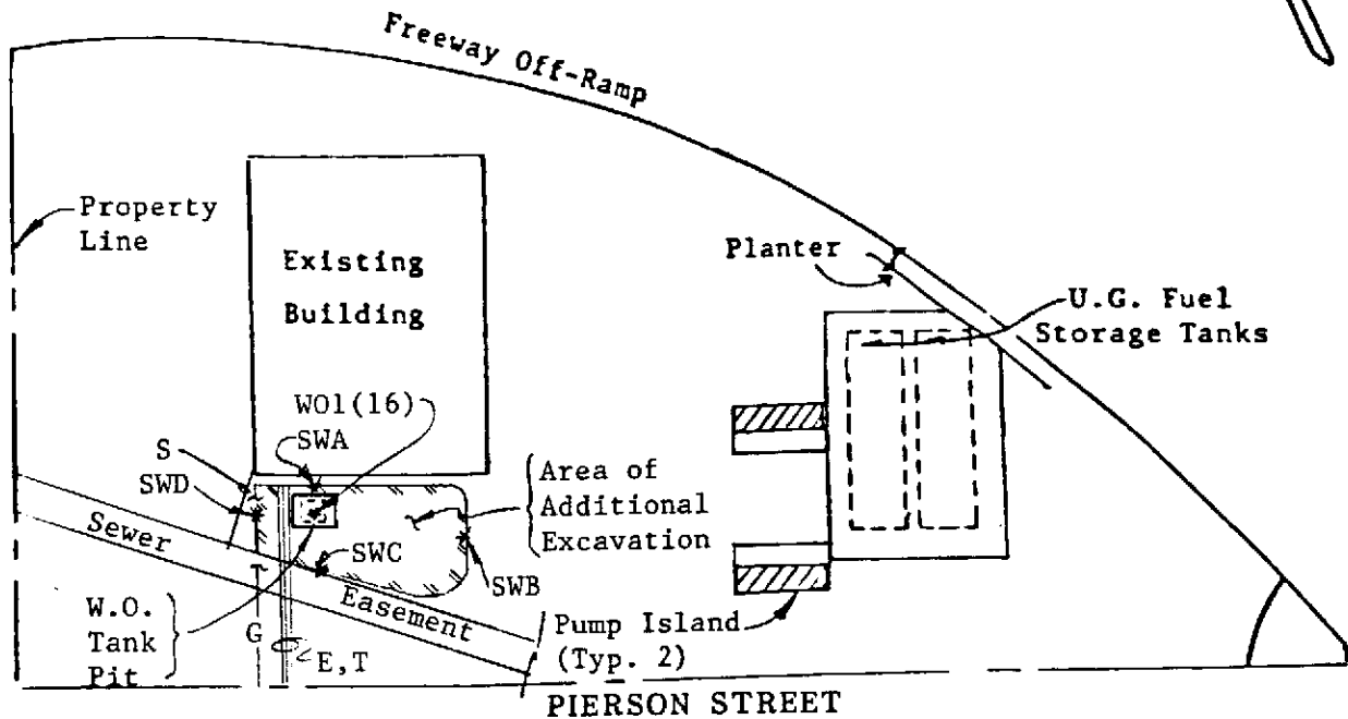
SITE PLAN
