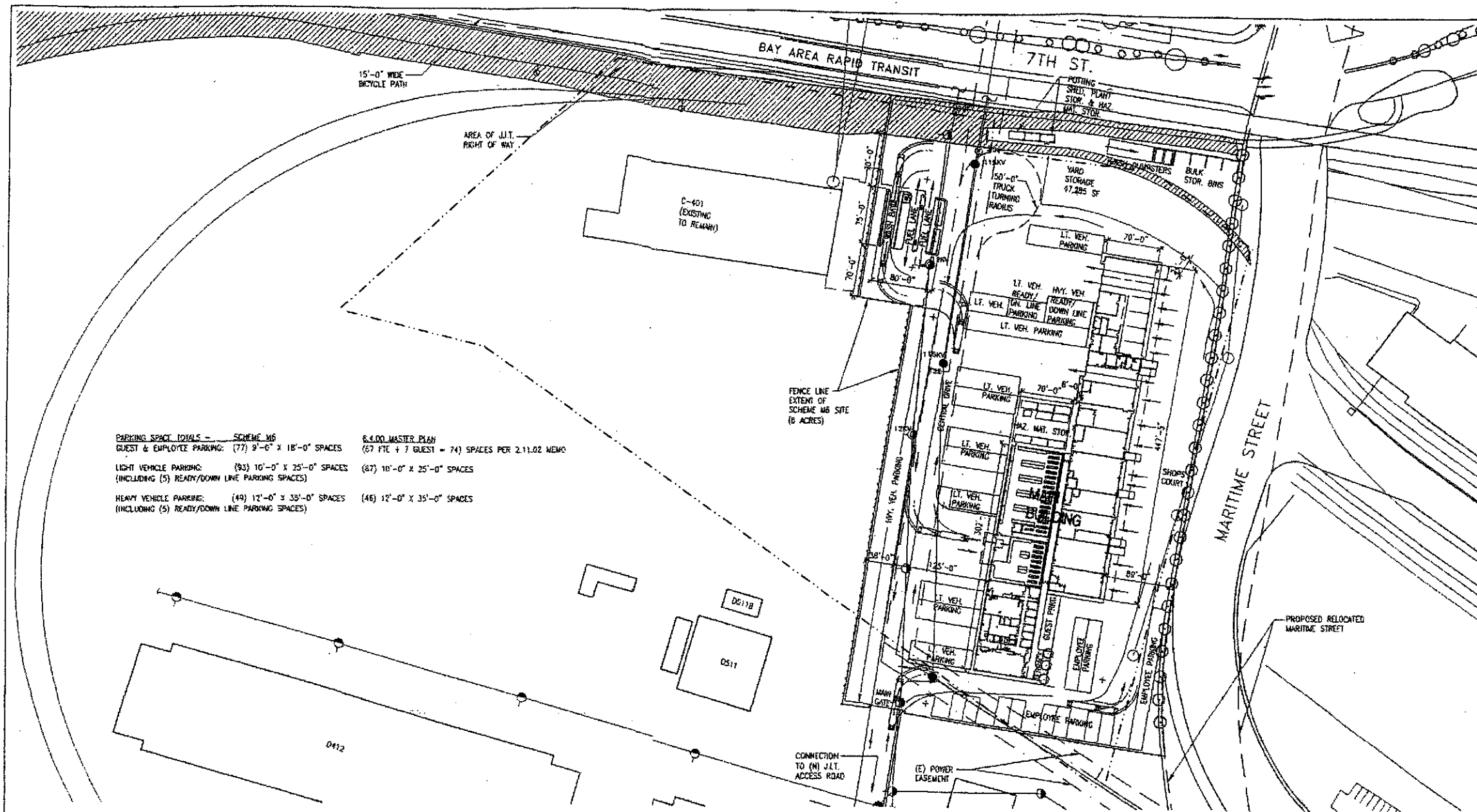
1 SITE PLAN - SCHEME M6 SCALE: 1" = 80'-0"
