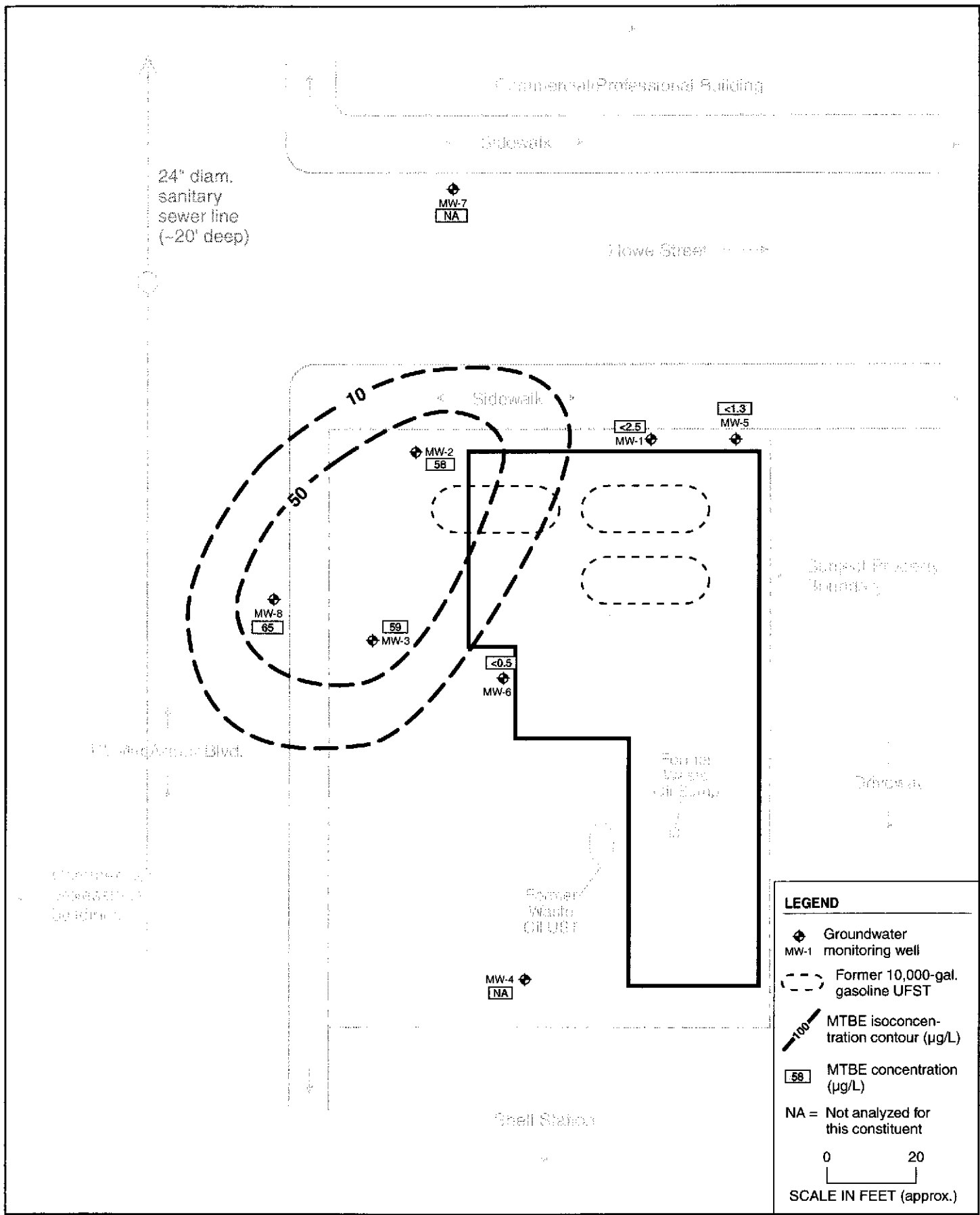
MTBE ISOCONCENTRATION CONTOURS (SEPTEMBER 2005)
