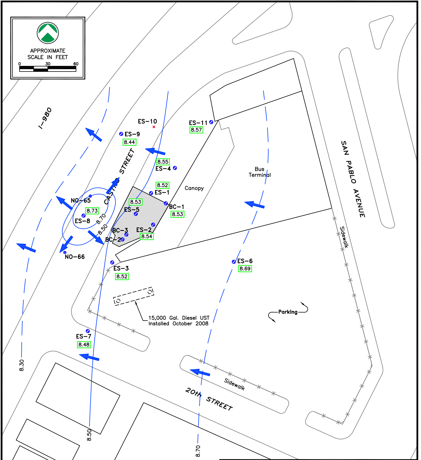
FIGURE 3 GROUNDWATER GRADIENT (February 8, 2011)
