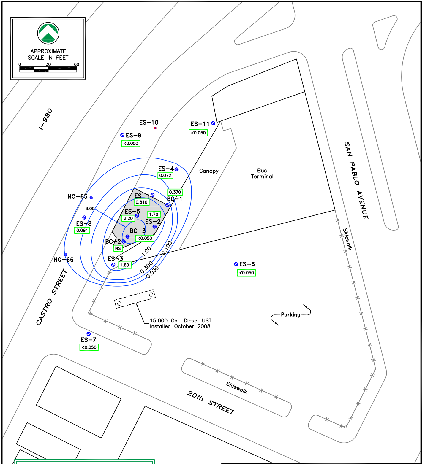
FIGURE 6 DISSOLVED-PHASE TPH-d IN GROUNDWATER (February 2011)
