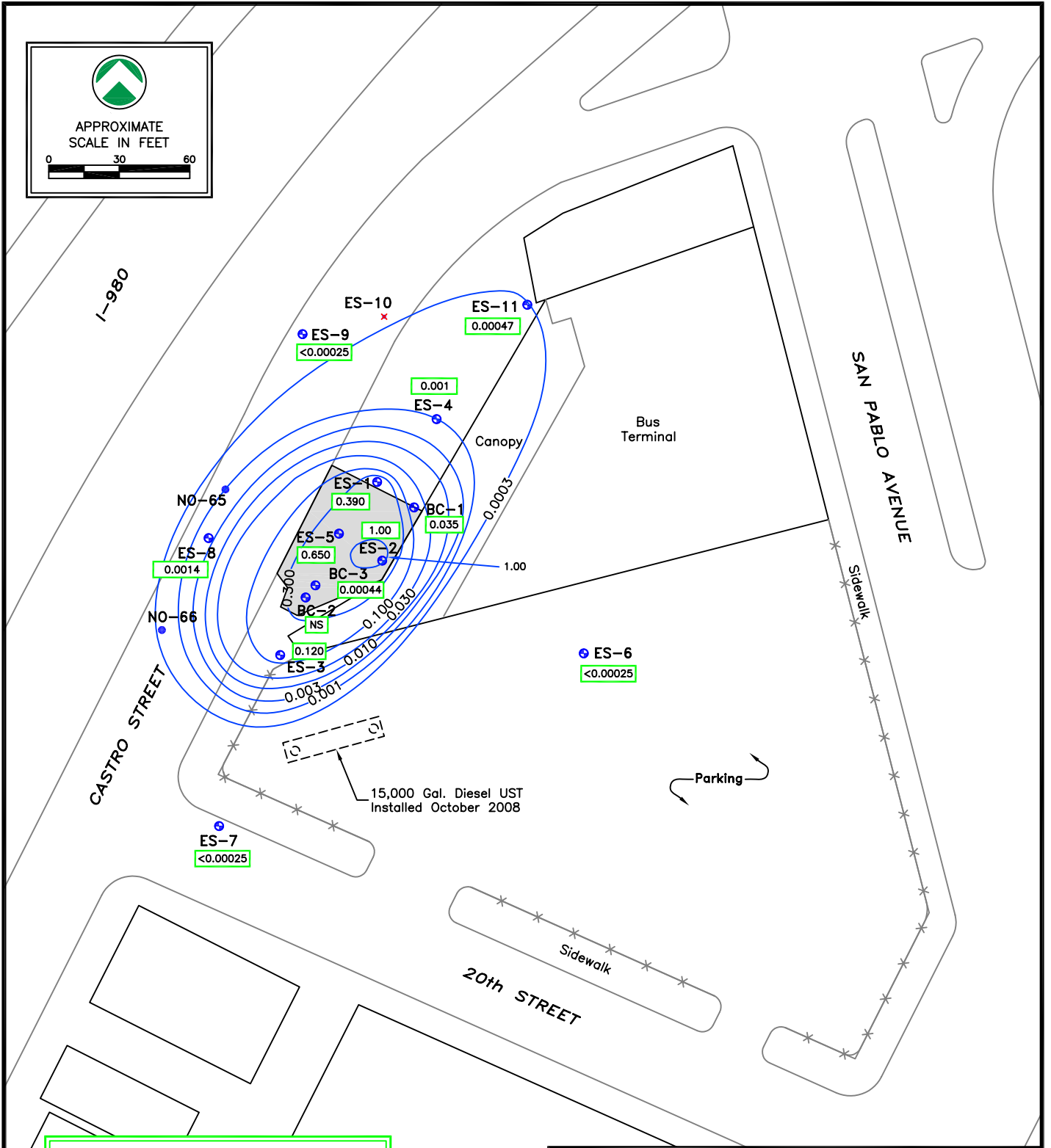
FIGURE 4 DISSOLVED-PHASE BENZENE IN GROUNDWATER (February 2011)
