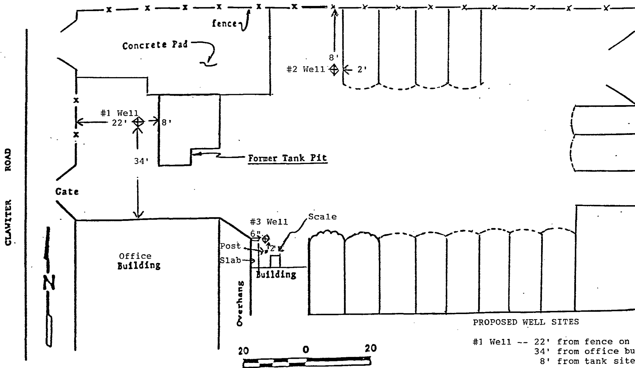
SITE PLAN
