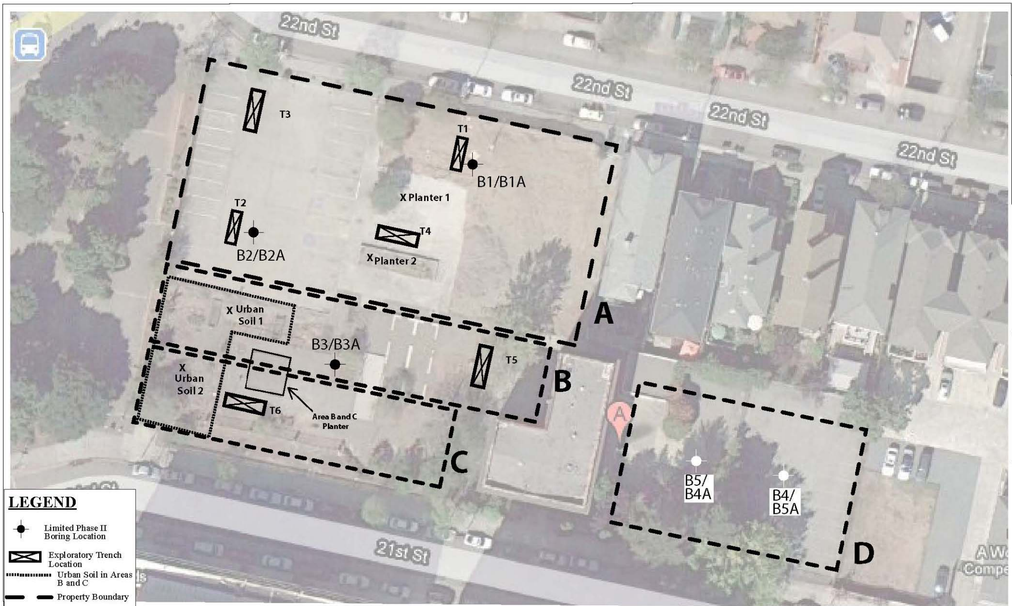
Figure 2 Site Plan Aerial Photograph Showing Lead-Impacted Soil in Areas B and C 2100 Martin Luther King Jr. Way 616-634 21st Street and 635 22nd Street Oakland, California
