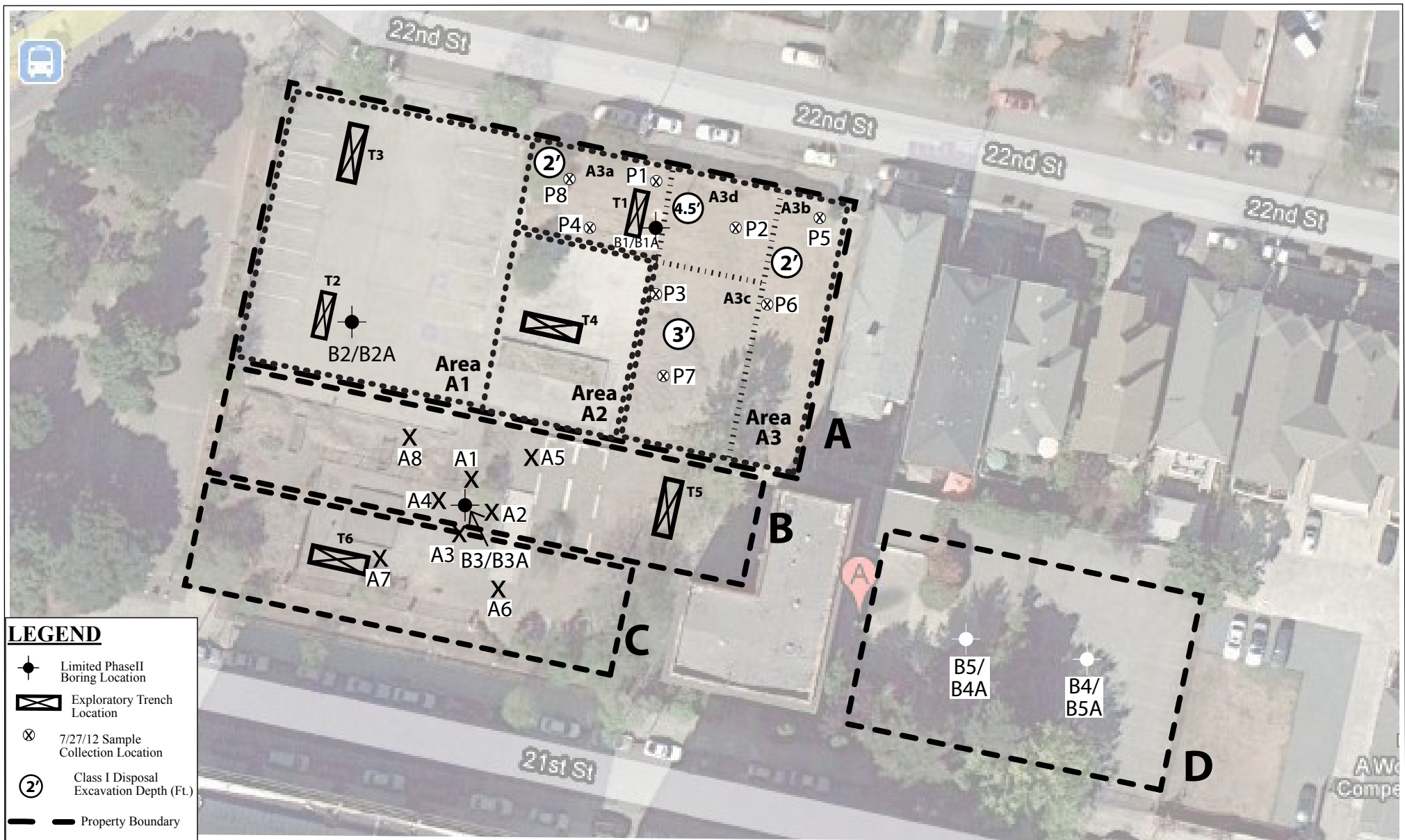
Figure 1 Site Plan Detail Showing Area Designations and Sample Collection Locations 2100 Martin Luther King Jr. Way 616-634 21st Street and 635 22nd Street Oakland, California
