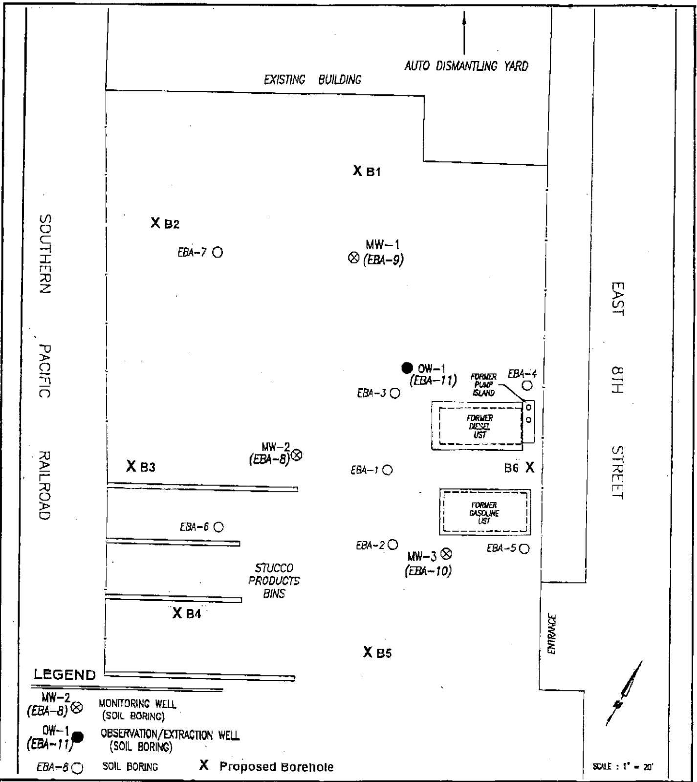
FIGURE 2 SITE PLAN Western Stucco Products 5115 East Eighth, Oakland, California
