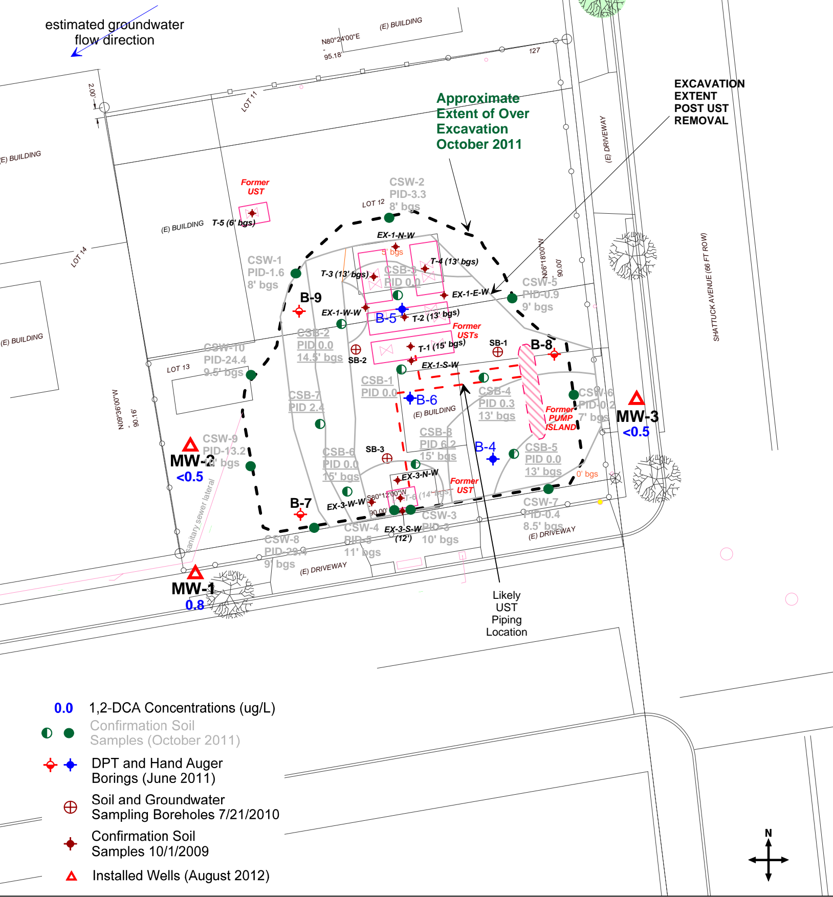
Figure 4: Map showing 1,2-DCA concentrations in groundwater, September 5, 2013
