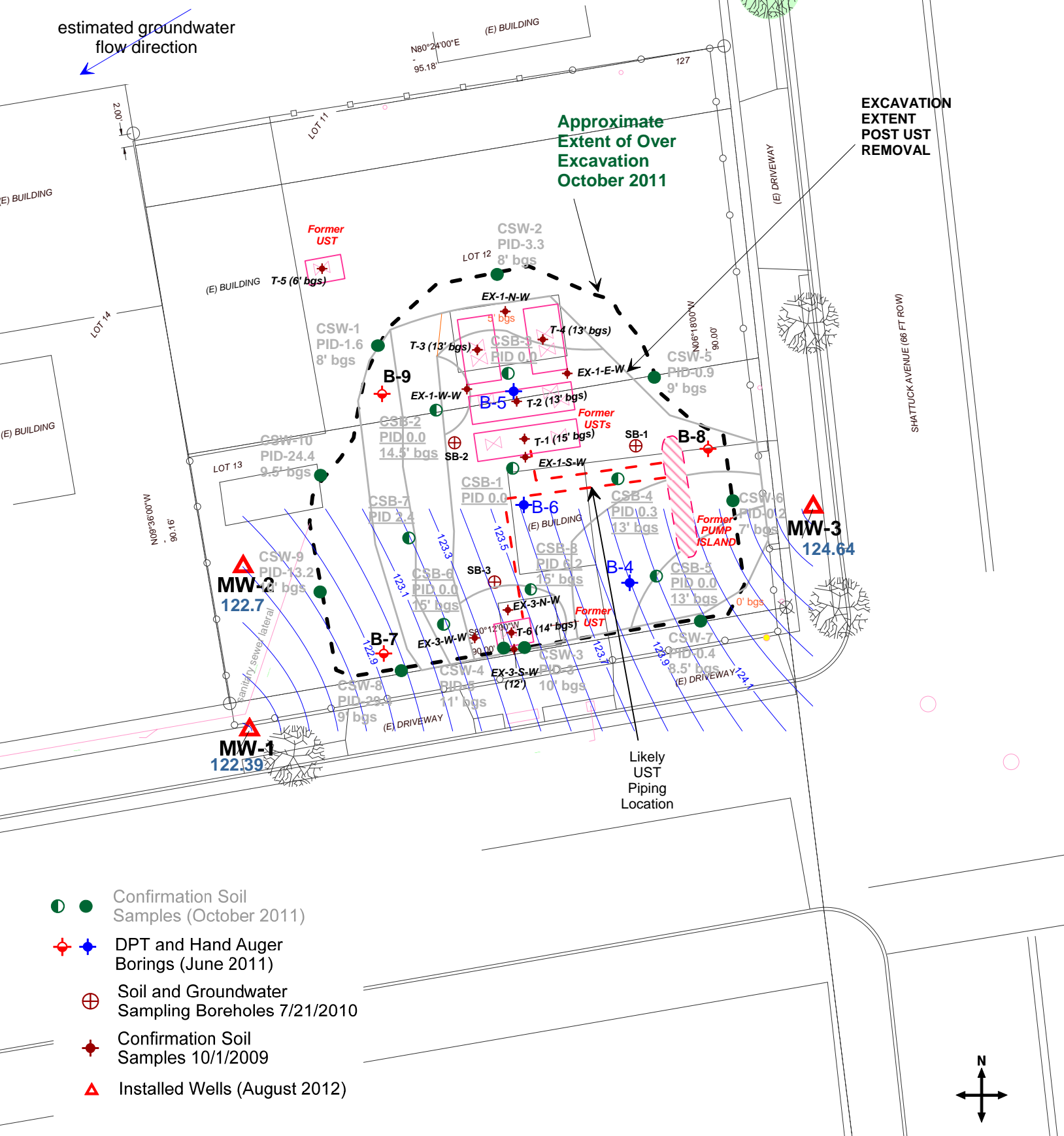
Figure 3: Groundwater elevation contour map in feet, September 5, 2013
