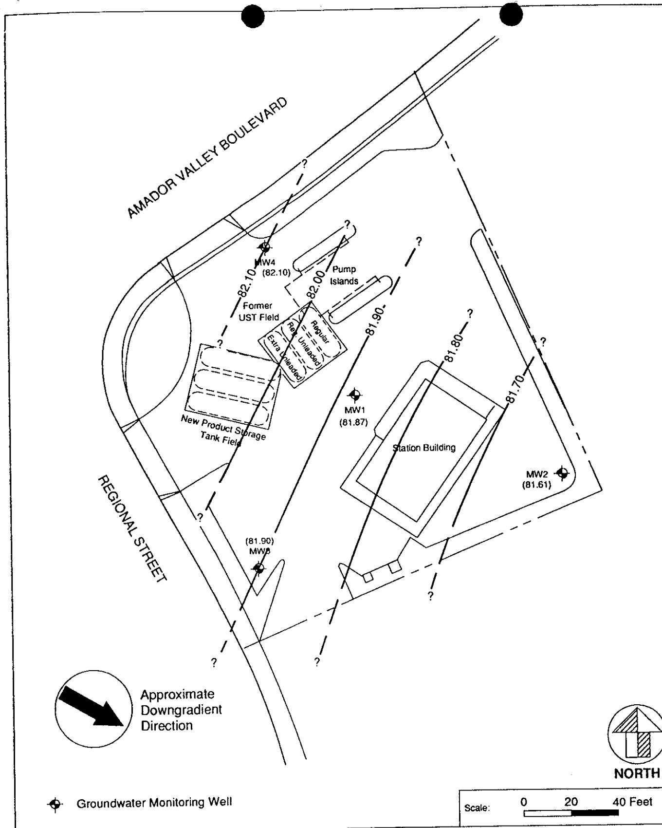
Figure 1. Elevations of groundwater (in feet, relative to a common datum) and indicated approximate direction of hydraulic gradient, Exxon RS 7-0210, Dublin, California, 21 May 1992.
