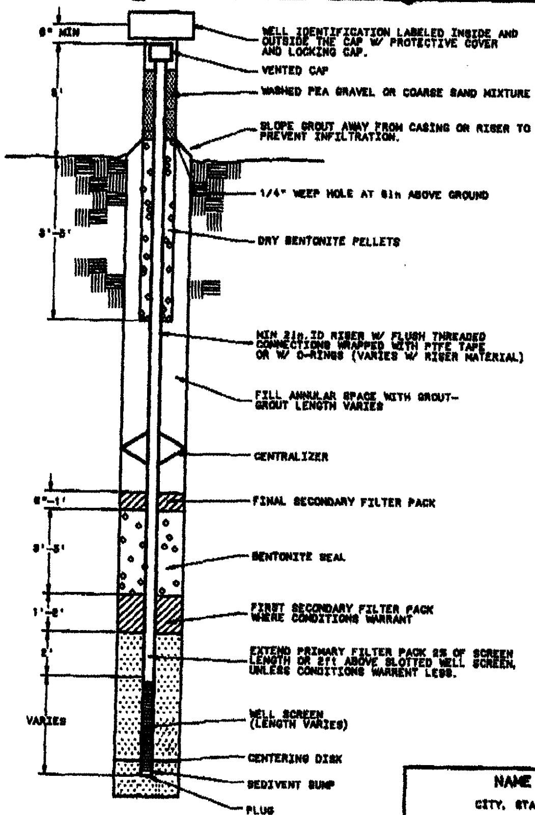
Single-Cased Monitoring Well - Non-Traffic Area
