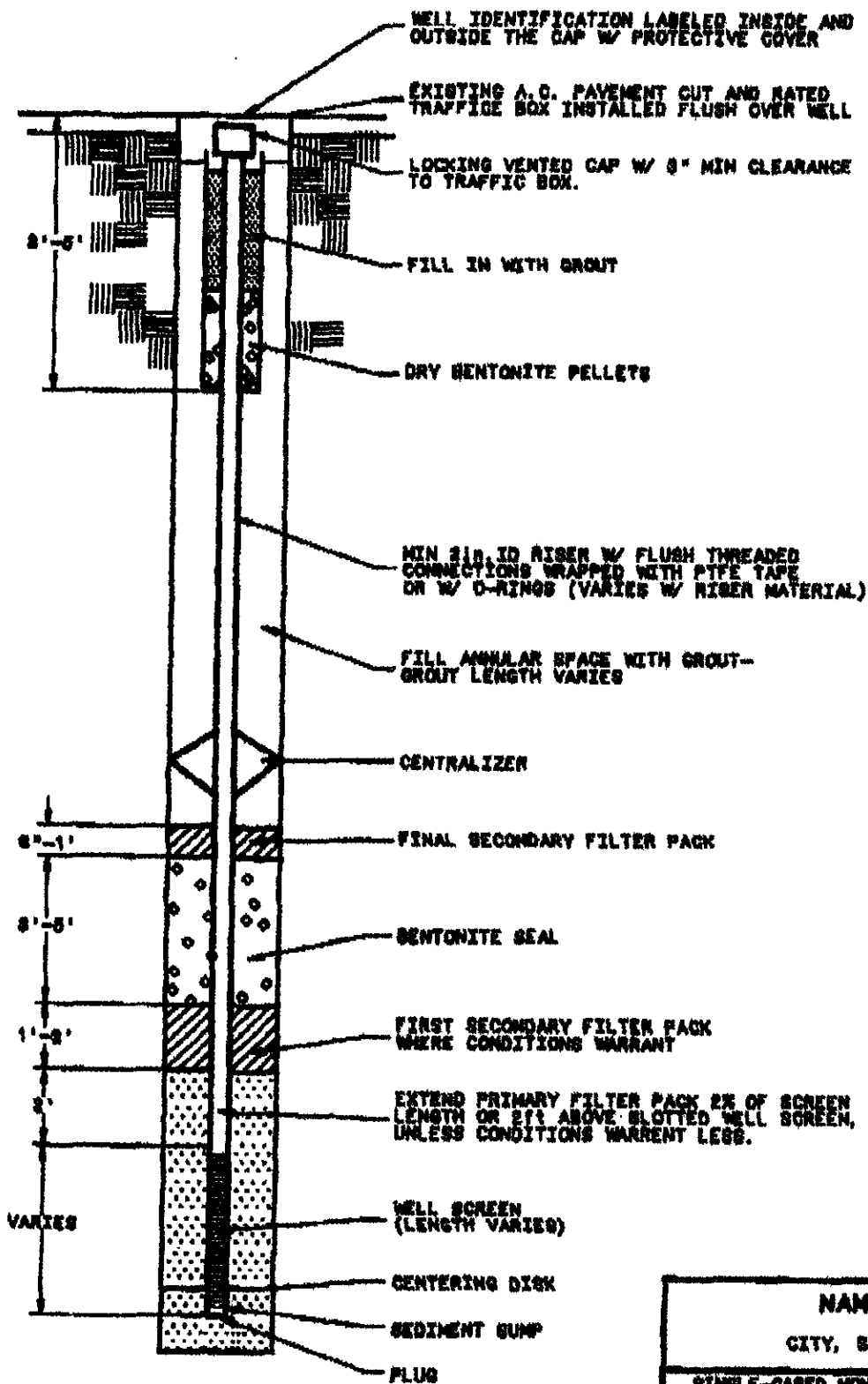
Single-Cased Monitoring Well - Paved Area
