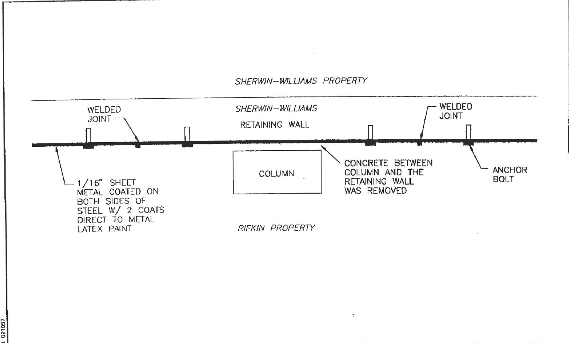
SHERWIN-WILLIAMS PLAN RIFKIN WALL (TYPICAL) N.T.S. Levine-Fricke-Rocan Figure 1 Project No. 3042
