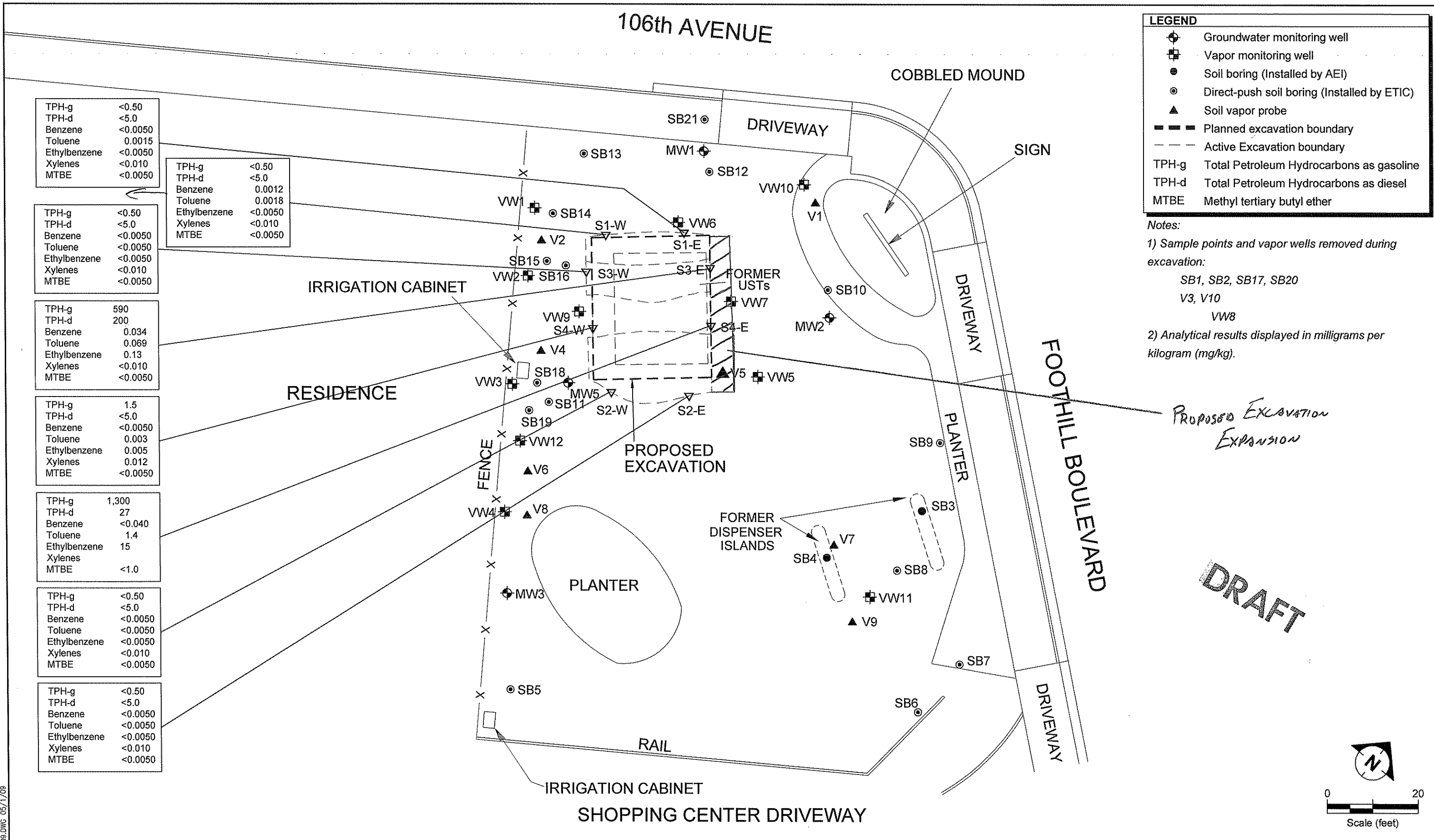
SITE MAP SHOWING EXTENT OF PROPOSED EXCAVATION FORMER EXXON RS 74121 10605 FOOTHILL BOULEVARD, OAKLAND, CALIFORNIA 27 MARCH AND 23 APRIL 2009
