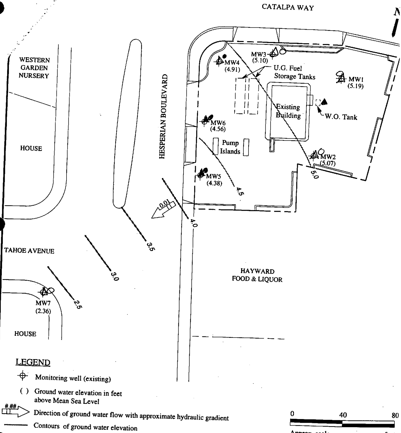
POTENTIOMETRIC SURFACE MAP FOR THE JULY 30, 1996 MONITORING EVENT
