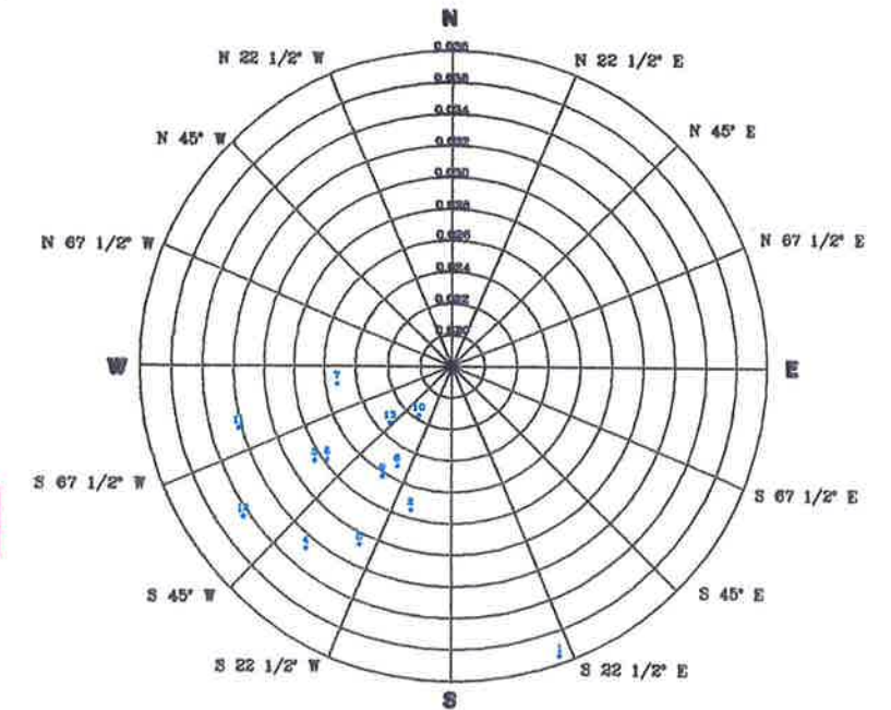
Compass Direction 13 Data Points Shown
