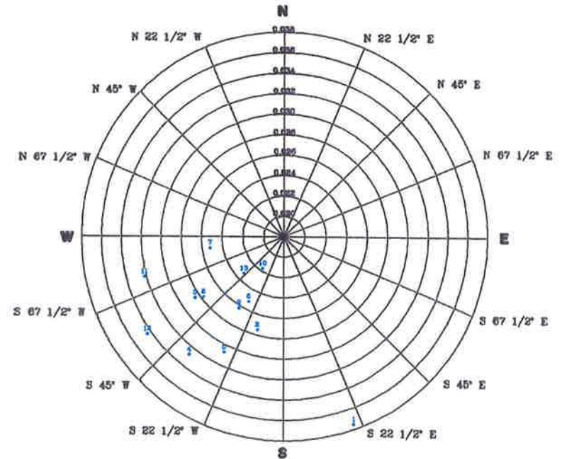
Compass Direction 13 Data Points Shown GROUNDWATER FLOW DIRECTION ROSE DIAGRAM
