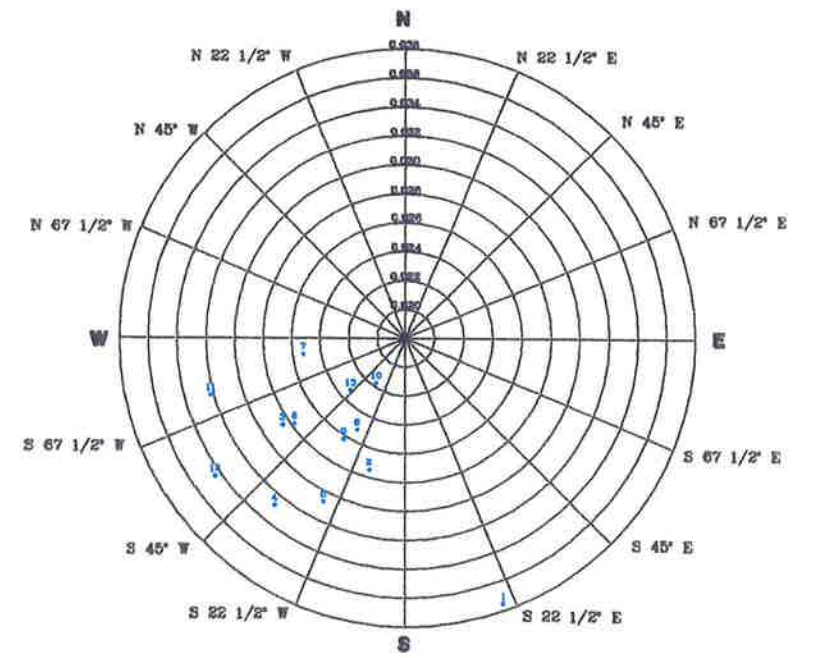
Compass Direction 13 Data Points Shown GROUNDWATER FLOW DIRECTION ROSE DIAGRAM
