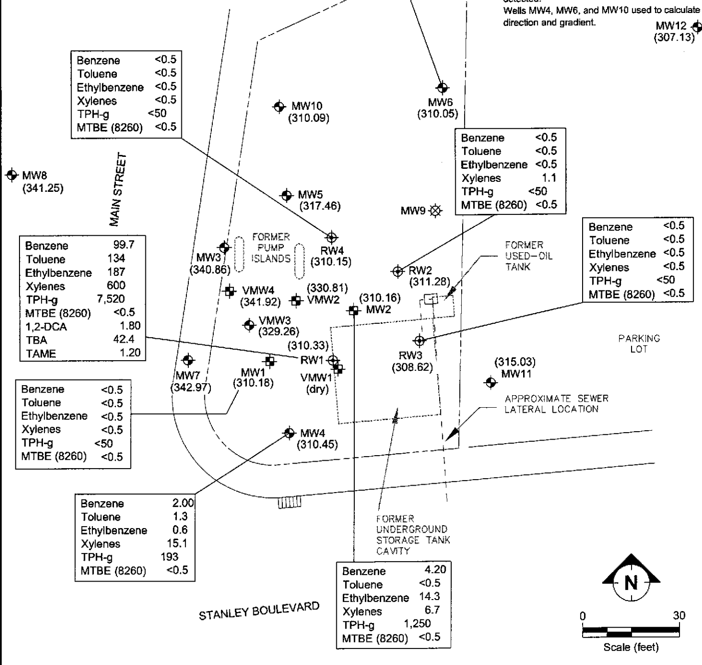
SITE PLAN SHOWING GROUNDWATER ELEVATIONS AND ANALYTICAL RESULTS, FORMER MOBIL STATION 04-H6J 1024 MAIN STREET, PLEASANTON, CALIFORNIA 14 APRIL 2005
