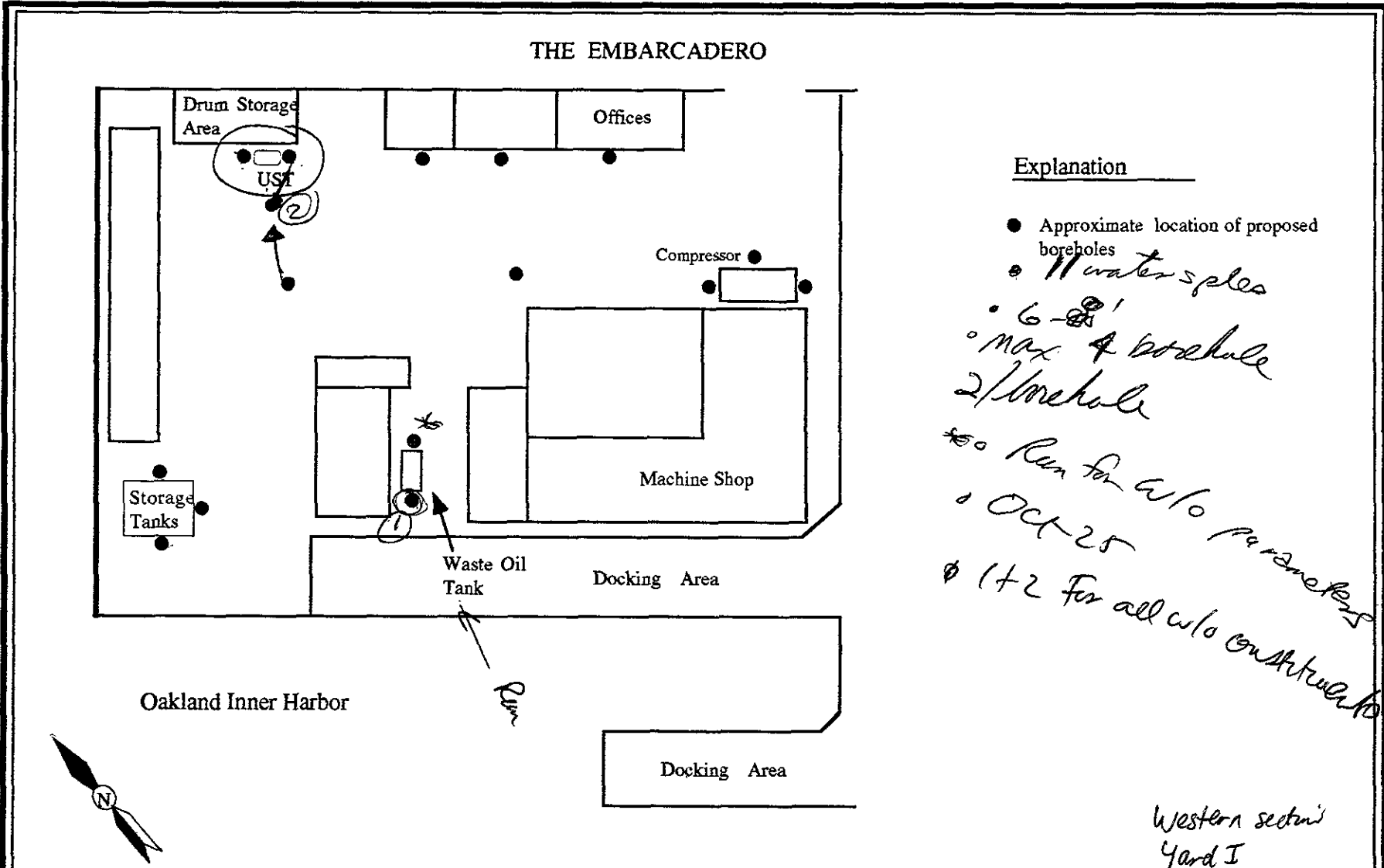
Figure 3-1. Location of Proposed Boreholes at Pacific Dry Dock Yard I
