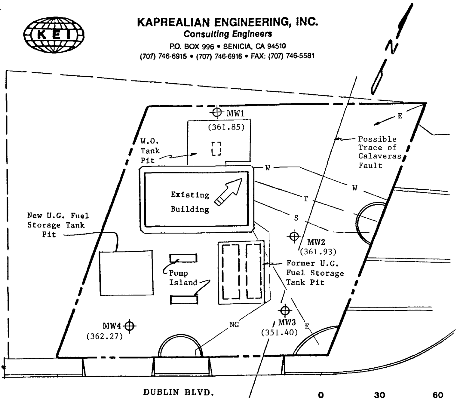
SITE PLAN Figure 1
