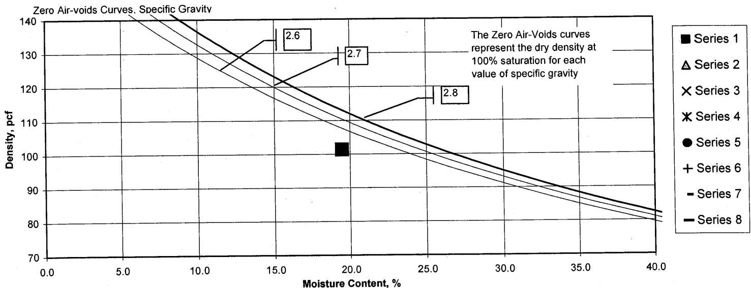
Moisture-Density
