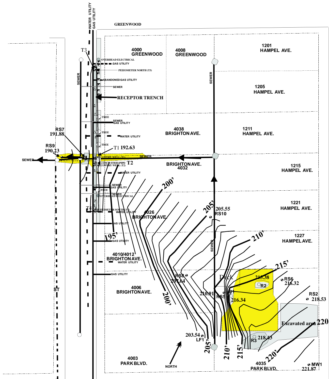
FIGURE 4 DP 793, 4035 PARK BLVD. OAKLAND, CALIFORNIA GROUNDWATER ELEVATION 06/21/2006.
