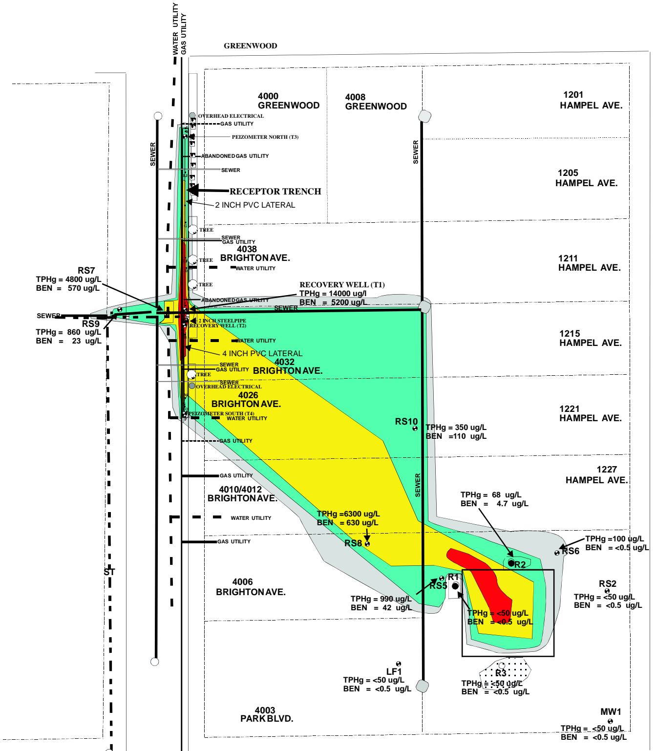
FIGURE 5 GROUNDWATER PLUME 06/21/06
