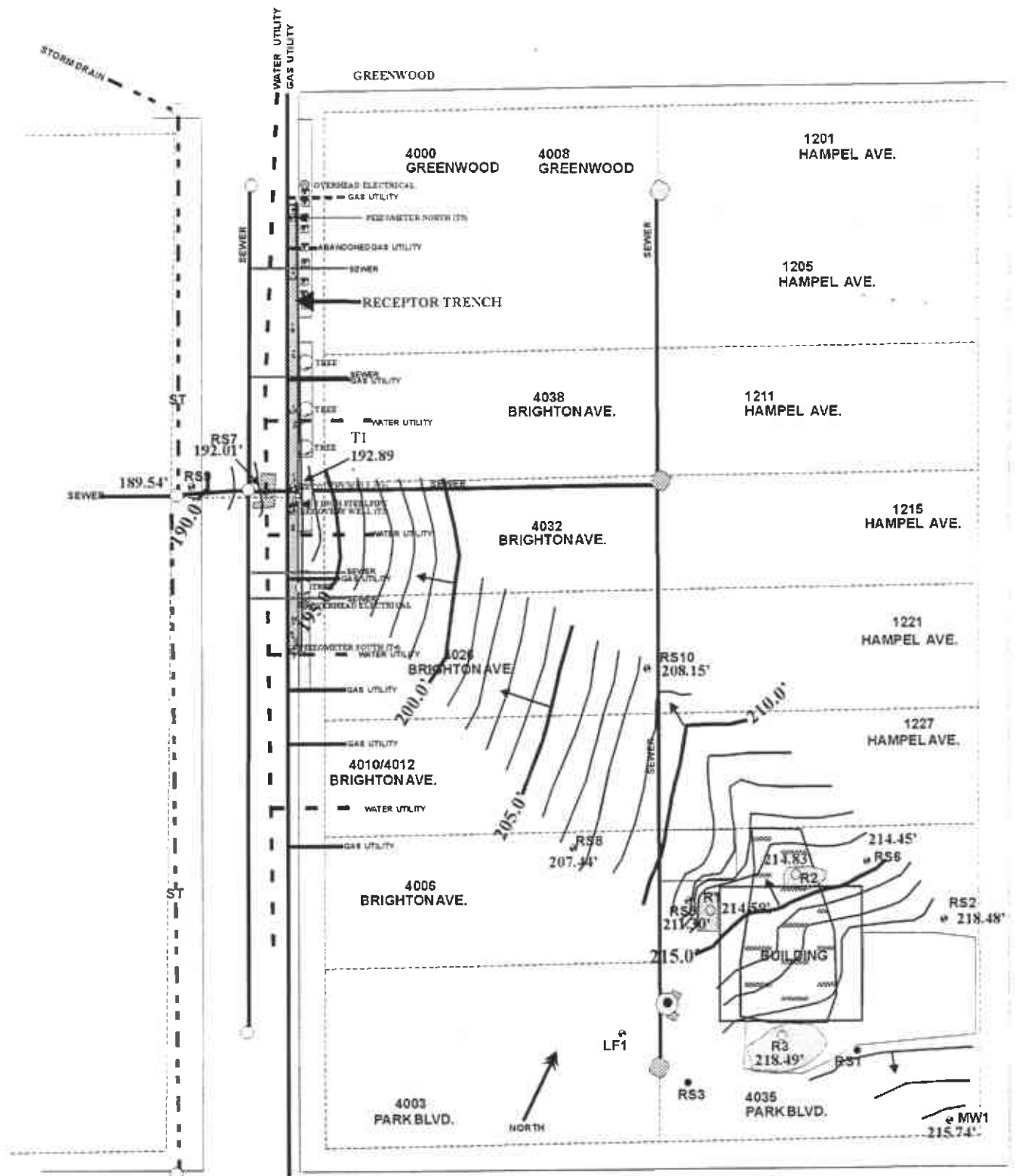
FIGURE 4 DP 793, 4035 PARK BLVD. OAKLAND, CALIFORNIA GROUNDWATER ELEVATION 02/09/00.
