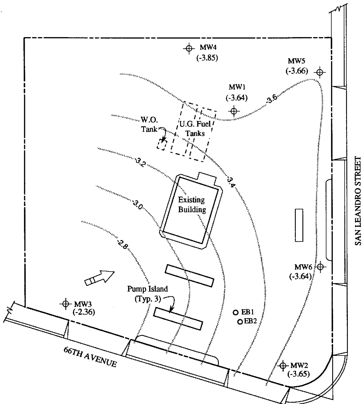
SITE PLAN
