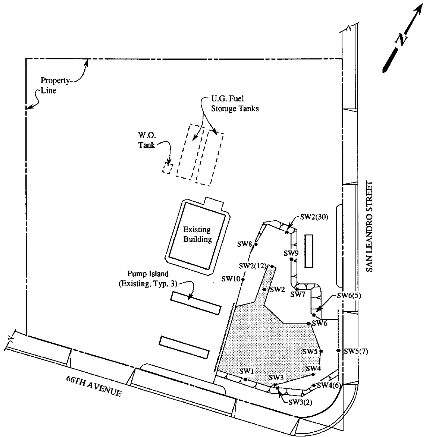
SITE PLAN
