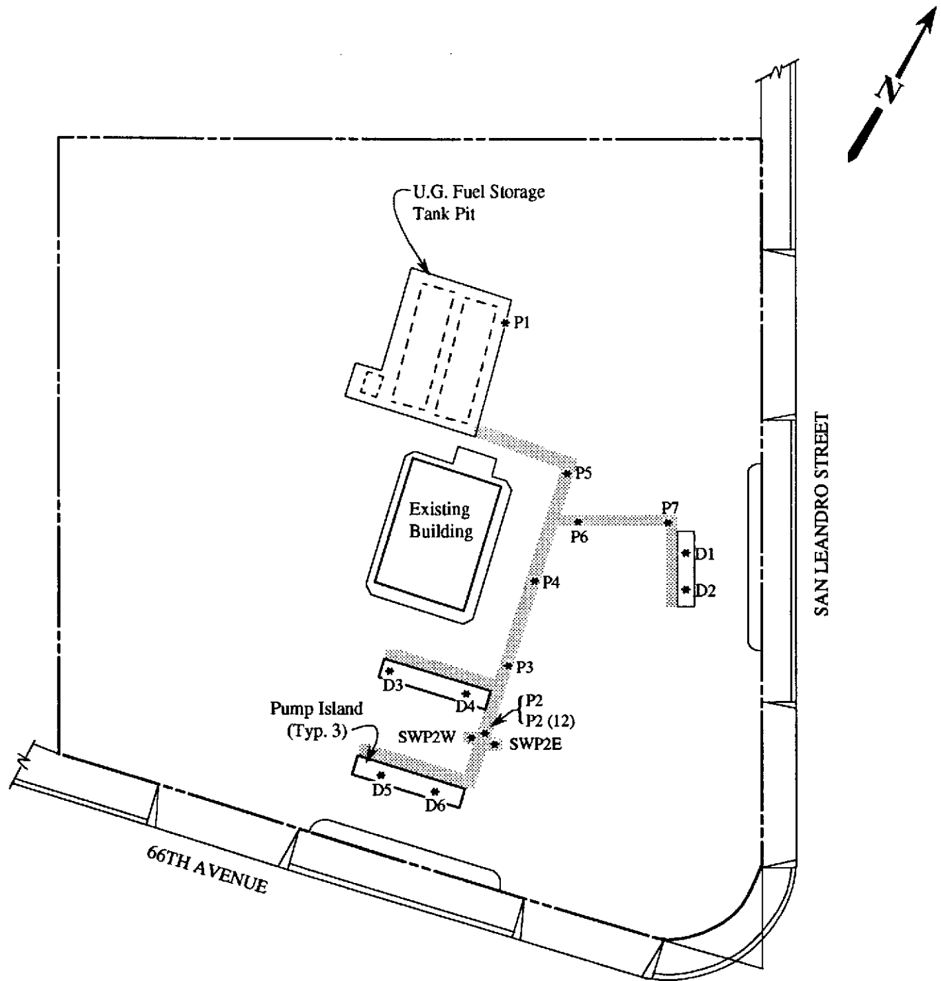
SITE PLAN
