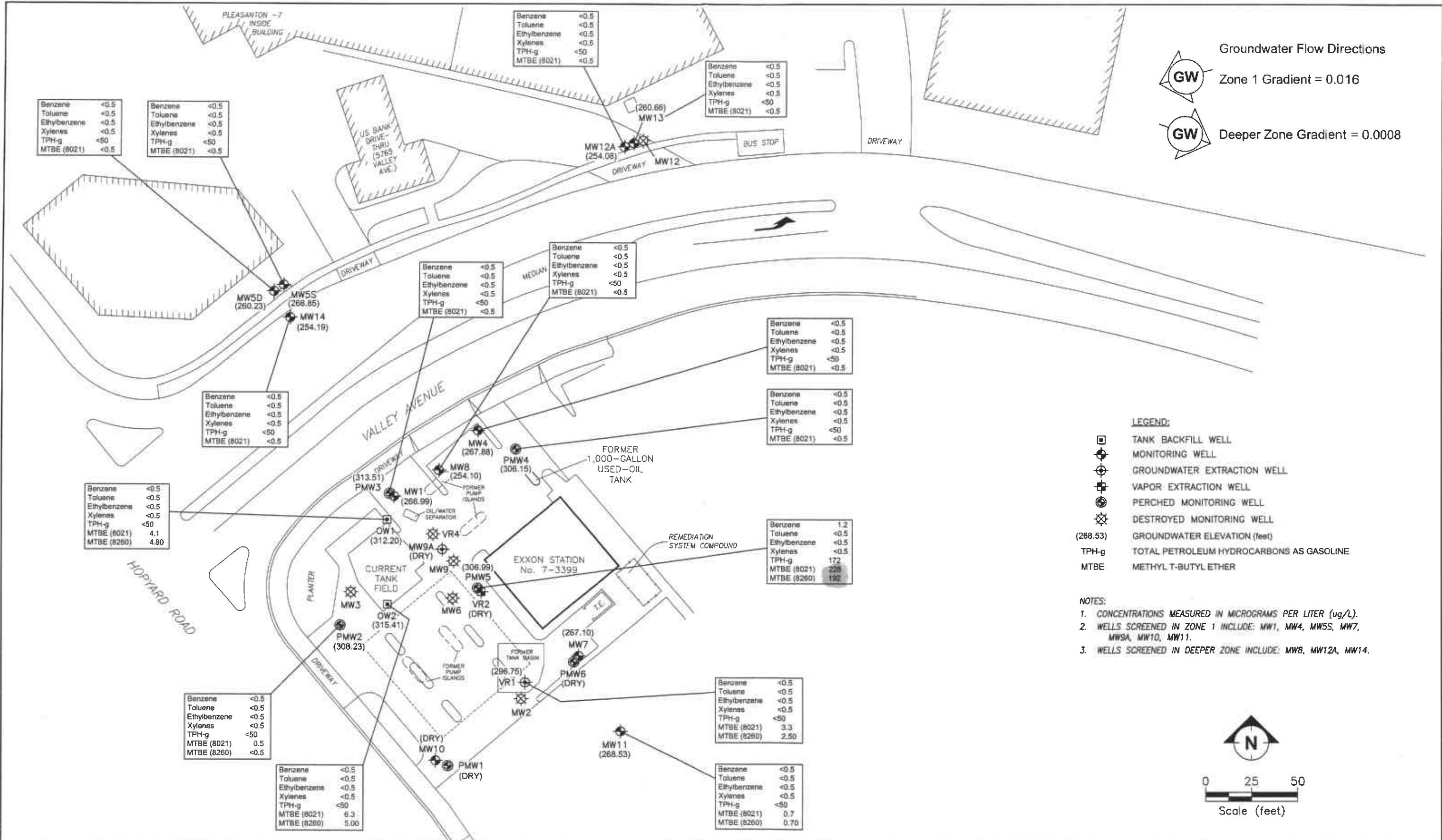
SITE PLAN SHOWING GROUNDWATER ELEVATIONS AND ANALYTICAL RESULTS FORMER EXXON RS 7-3399 2991 HOPYARD ROAD, PLEASANTON, CALIFORNIA 17 DECEMBER 2002
