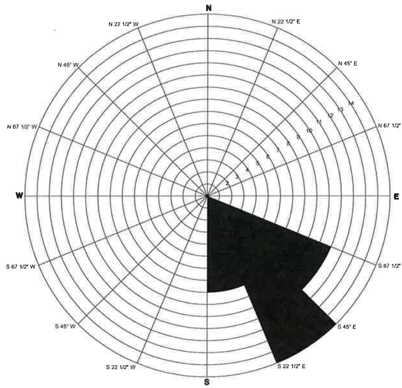
GROUNDWATER FLOW DIRECTION ROSE DIAGRAM Second Quarter 2003-Fourth Quarter 2013
