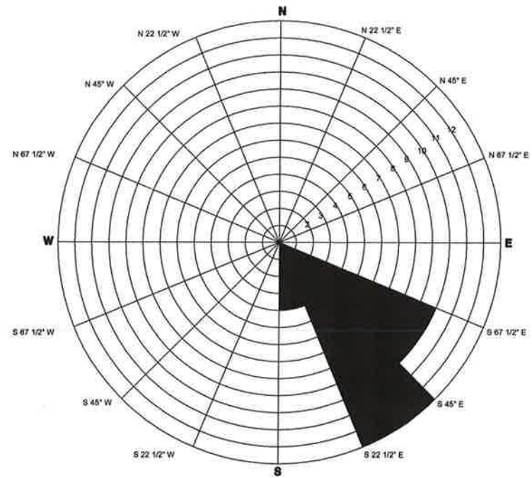
GROUNDWATER FLOW DIRECTION ROSE DIAGRAM Second Quarter 2003-First Quarter 2010
