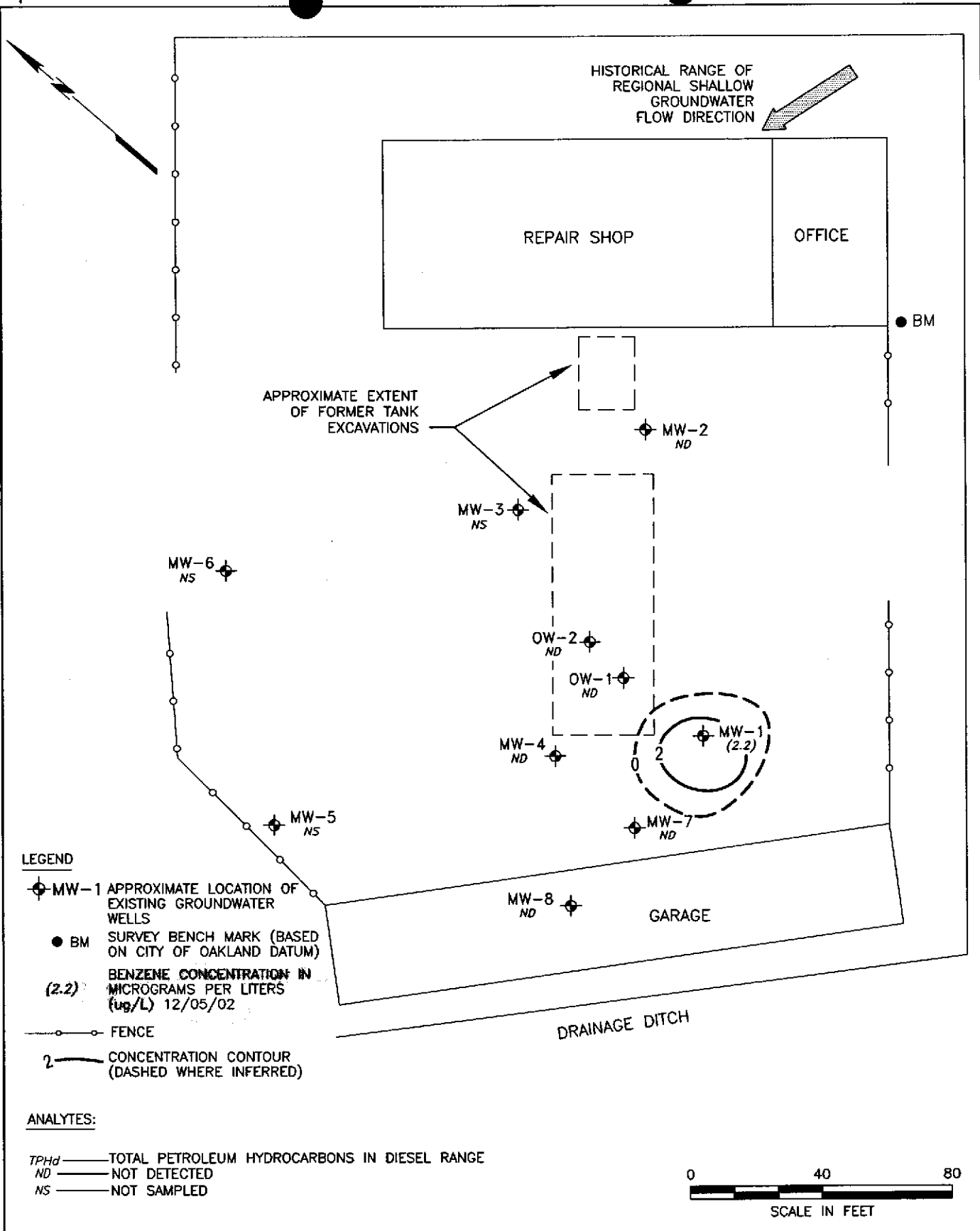
FIGURE 5 FORMER PENSKE TRUCKING COMPANY 725 JULIE ANN WAY OAKLAND, CALIFORNIA BENZENE CONCENTRATIONS IN GROUNDWATER
