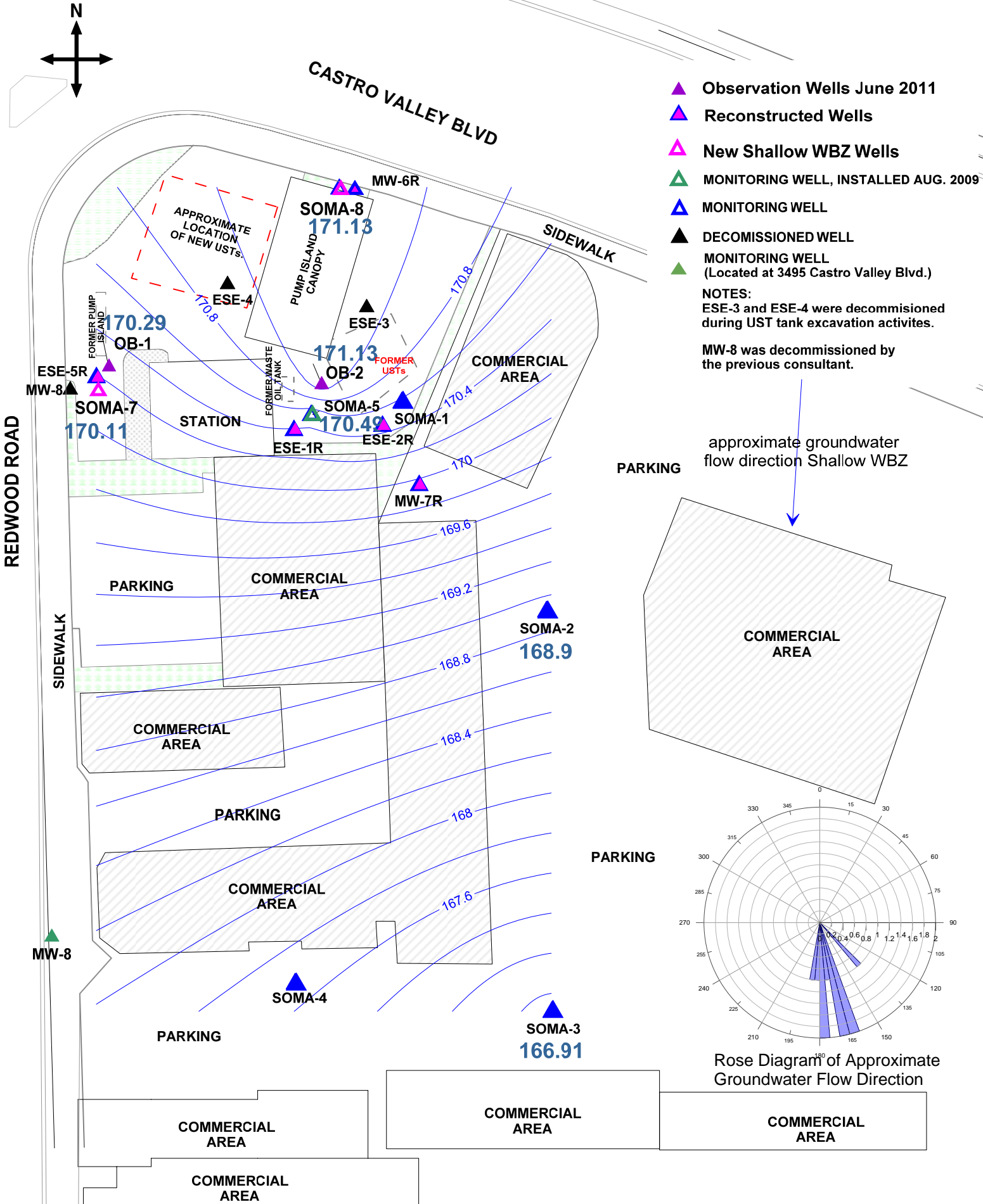
Figure 3: Groundwater Elevation Contour Map for Shallow WBZ Wells in Feet. January 19, 2015
