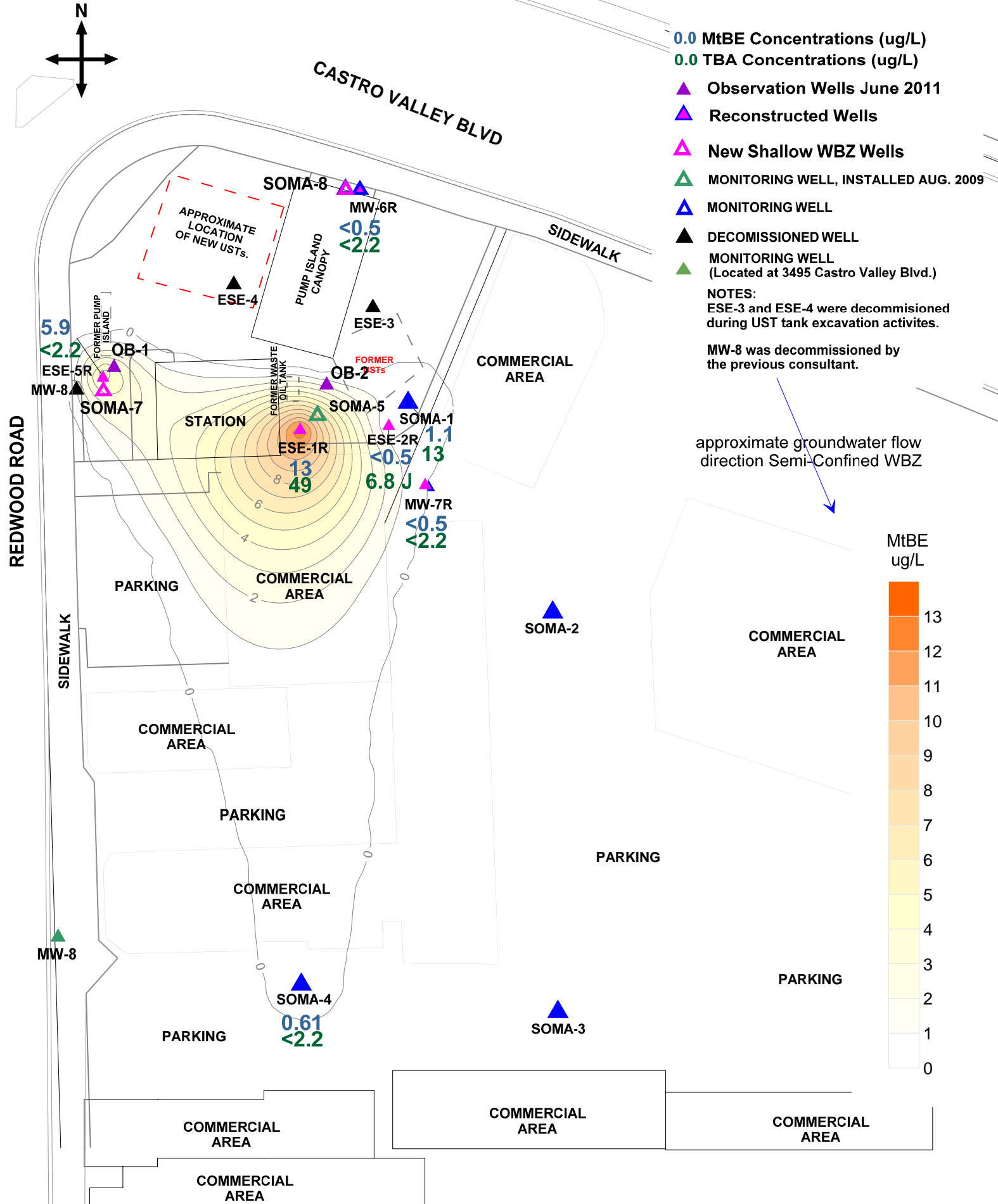
Figure 10: Contour Map of MtBE and Map of TBA Concentrations in Semi-Confined WBZ Wells. January 19 and 20, 2015
