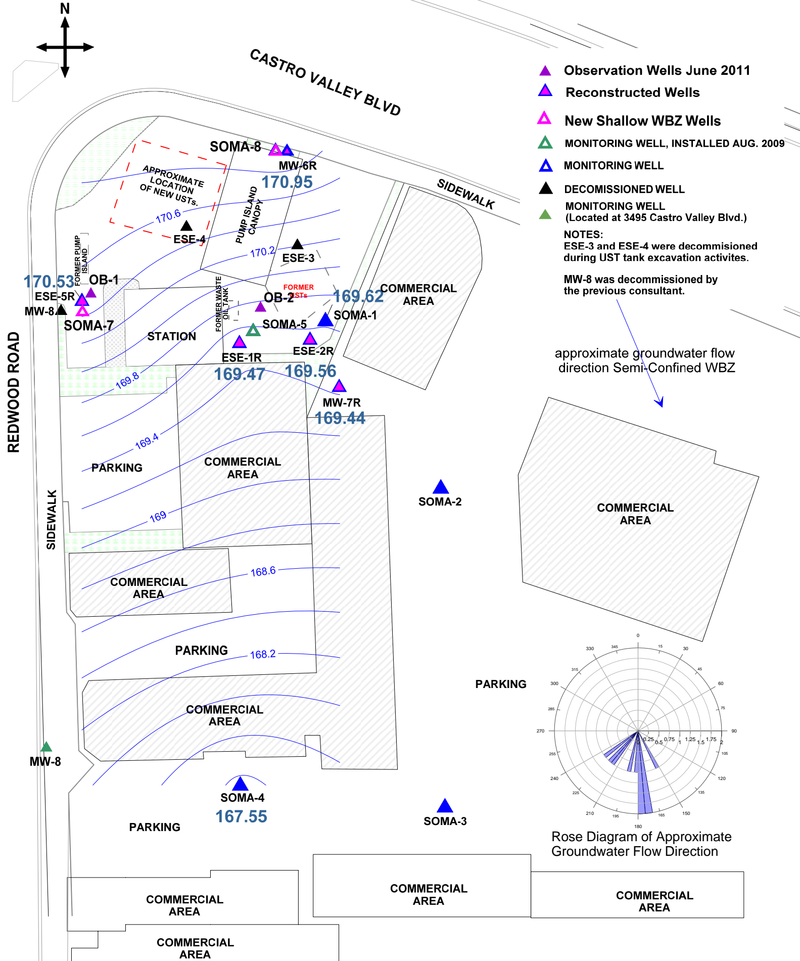
Figure 8: Groundwater Elevation Contour Map for Semi-Confined WBZ Wells in Feet. January 19, 2015
