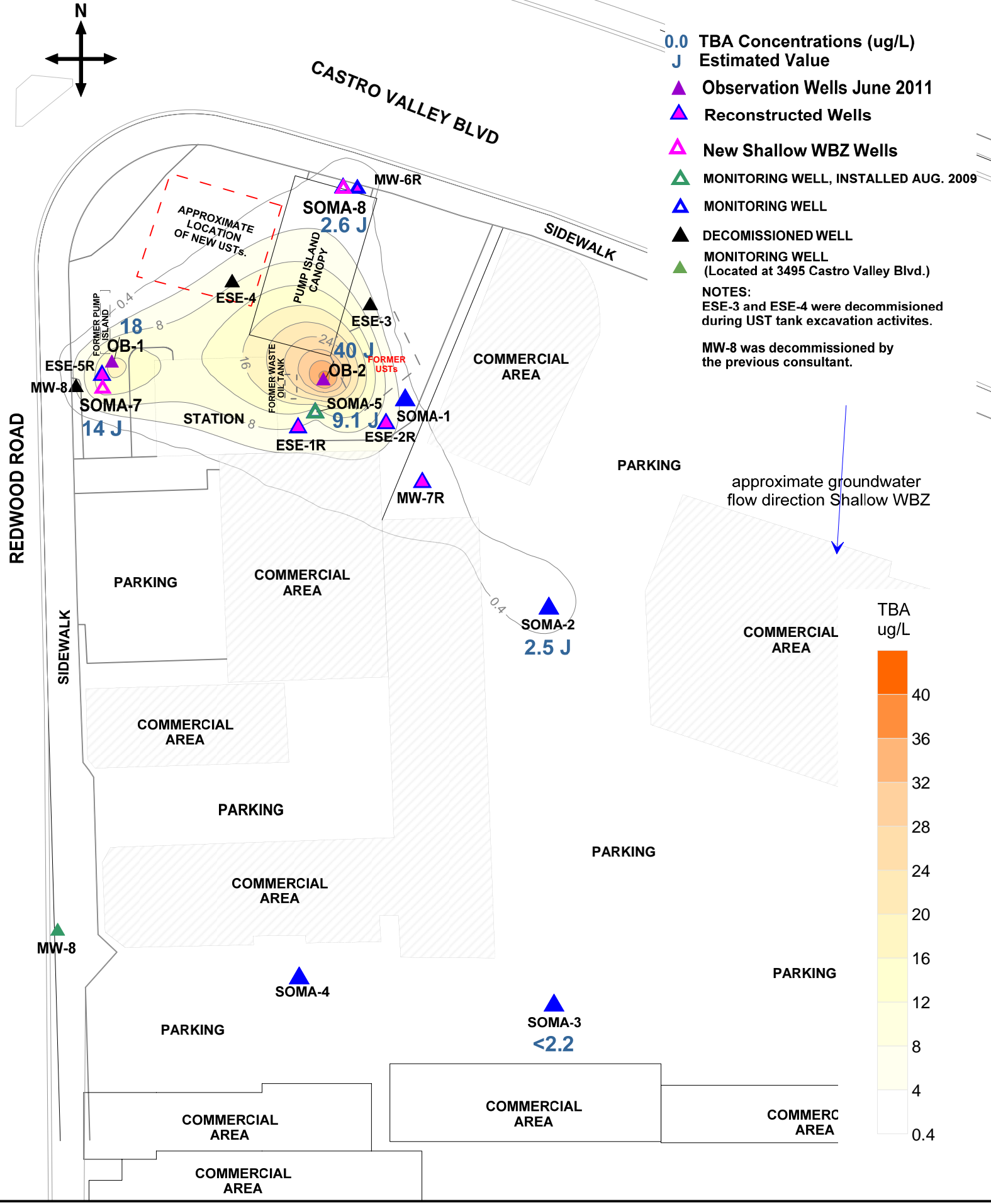
Figure 7: Contour Map of TBA Concentrations in Shallow WBZ Wells in Feet. January 19 and 20, 2015
