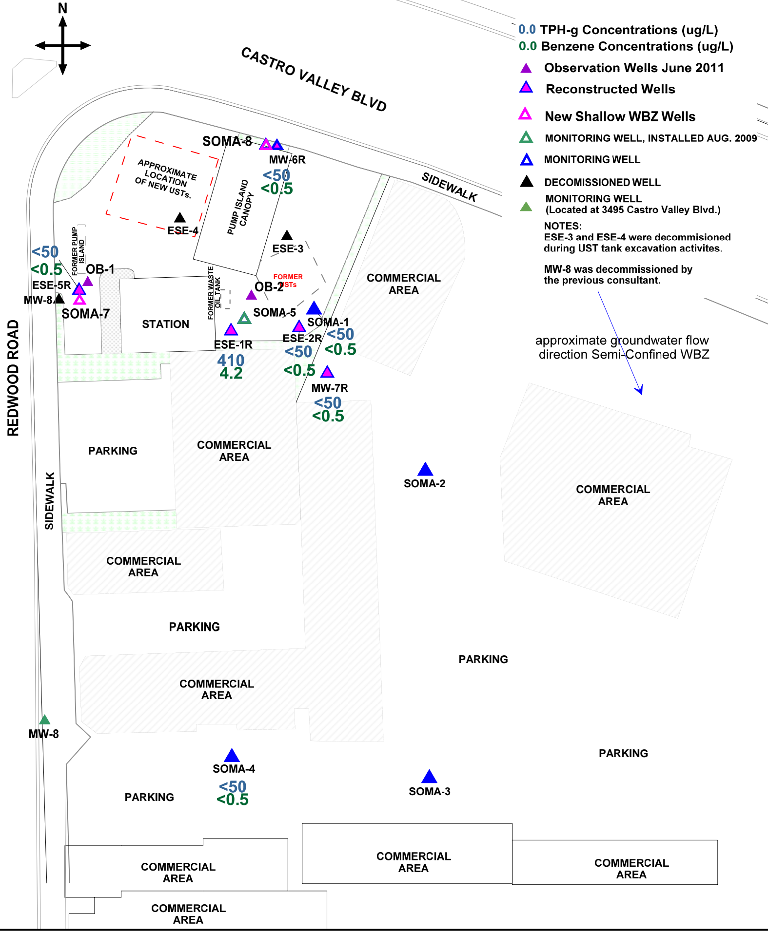
Figure 9: Map of TPH-g and Benzene Concentrations in Semi-Confined WBZ Wells. January 19 and 20, 2015
